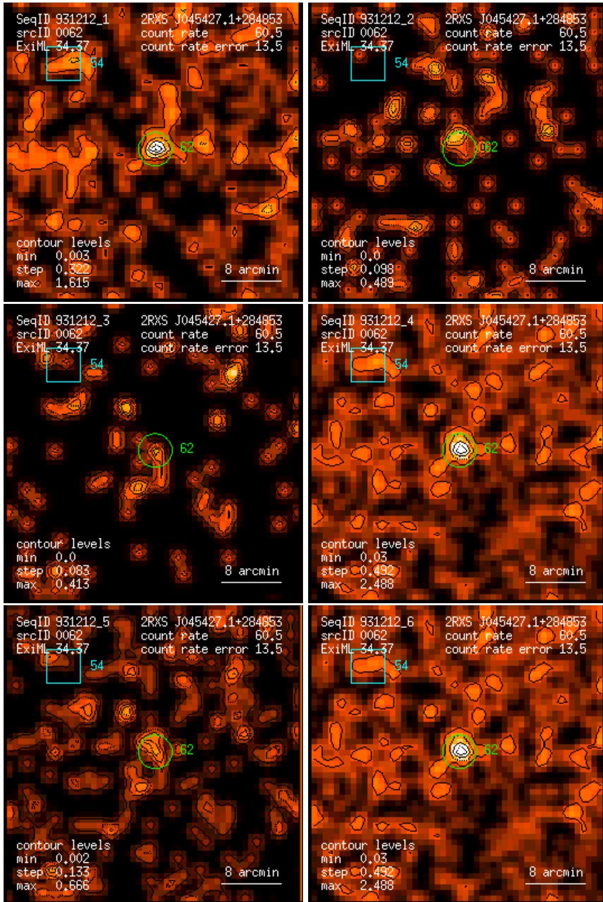
Figure 62: RASS 931212: detection 0062: band rate images, Gaussian filter: (1) PSPC channels 11 – 41, (2) 52 – 90, (3) 91 – 201, (4) 11 – 235, (5) 52 – 201, (6) 11 – 201. Broad band rates in counts/ks. Band rate contour levels in counts/ks/arcmin 2 .
