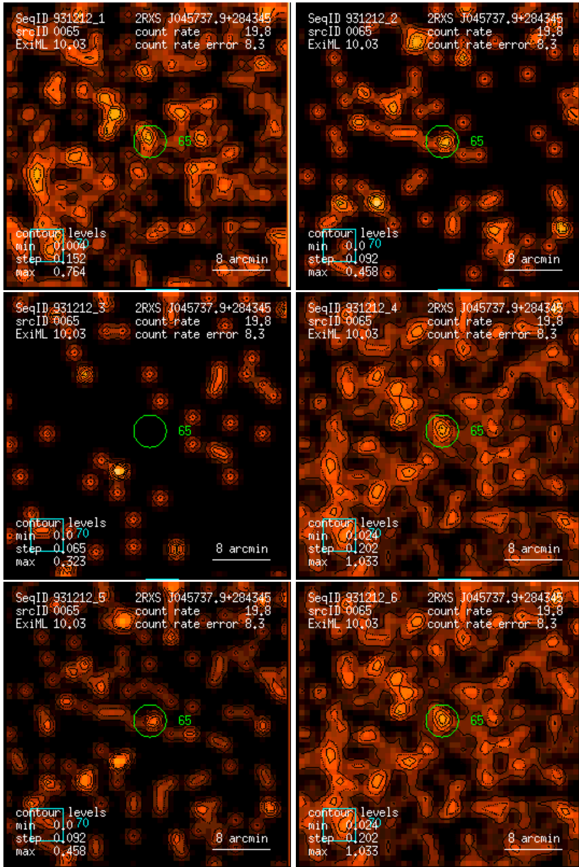
Figure 65: RASS 931212: detection 0065: band rate images, Gaussian filter: (1) PSPC channels 11 – 41, (2) 52 – 90, (3) 91 – 201, (4) 11 – 235, (5) 52 – 201, (6) 11 – 201. Broad band rates in counts/ks. Band rate contour levels in counts/ks/arcmin 2 .
