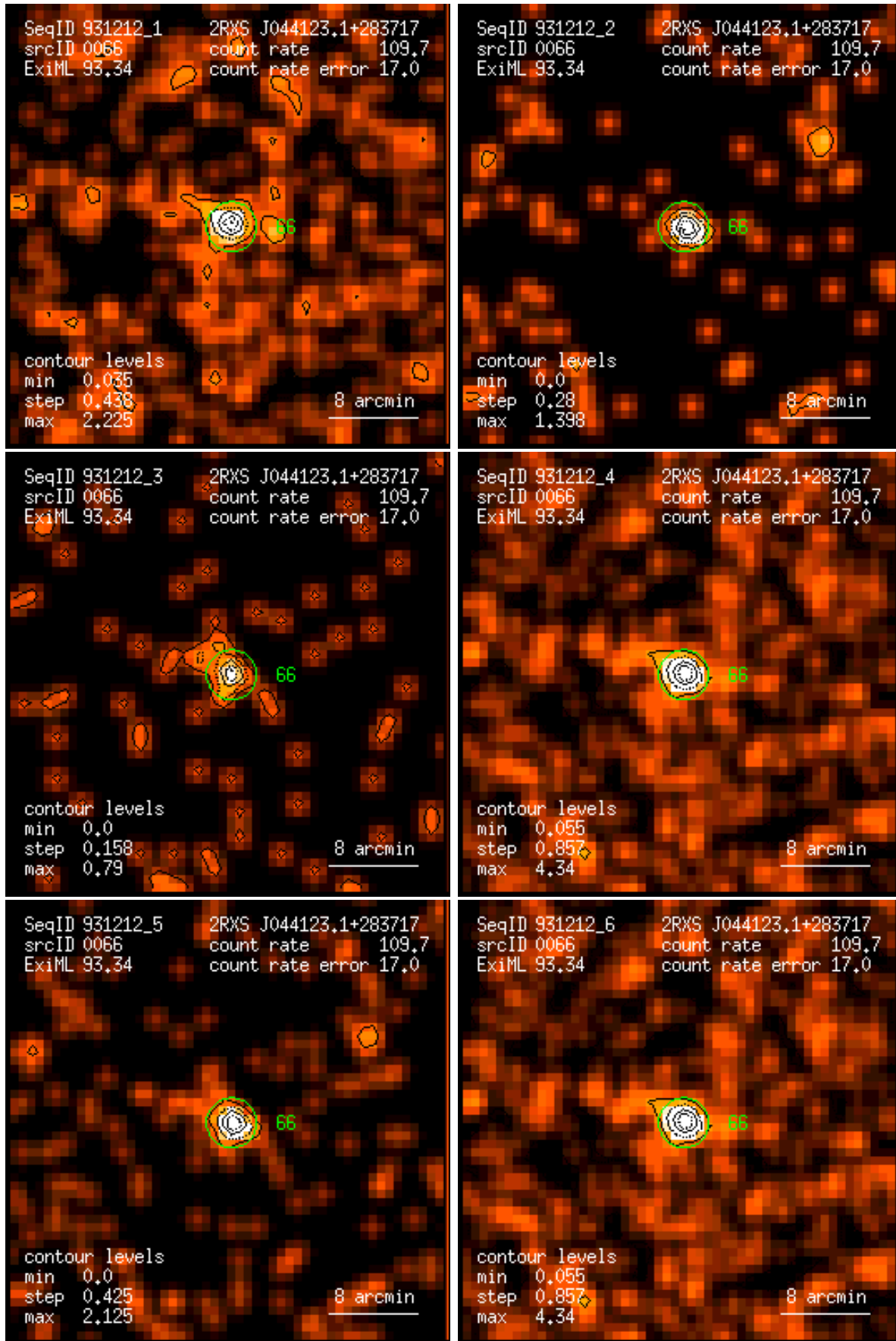
Figure 66: RASS 931212: detection 0066: band rate images, Gaussian filter: (1) PSPC channels 11 – 41, (2) 52 – 90, (3) 91 – 201, (4) 11 – 235, (5) 52 – 201, (6) 11 – 201. Broad band rates in counts/ks. Band rate contour levels in counts/ks/arcmin 2 .
