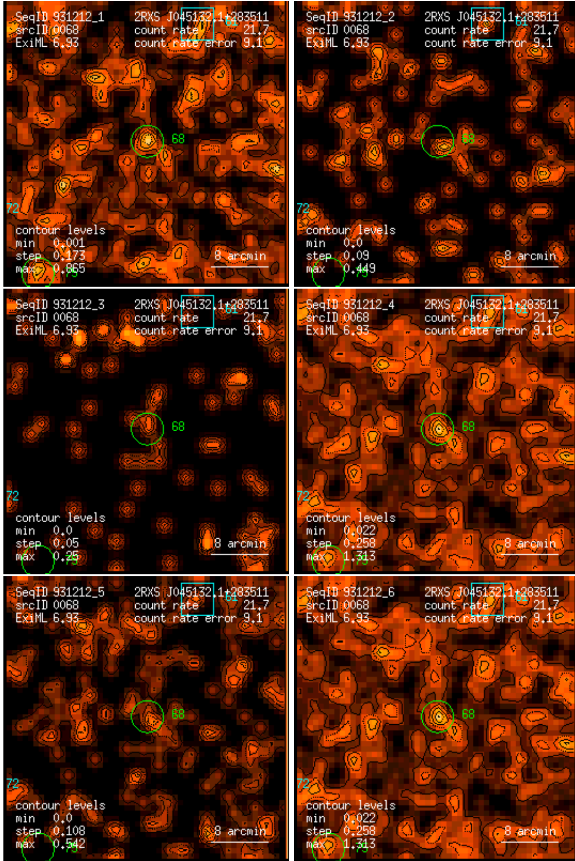
Figure 68: RASS 931212: detection 0068: band rate images, Gaussian filter: (1) PSPC channels 11 – 41, (2) 52 – 90, (3) 91 – 201, (4) 11 – 235, (5) 52 – 201, (6) 11 – 201. Broad band rates in counts/ks. Band rate contour levels in counts/ks/arcmin 2 .
