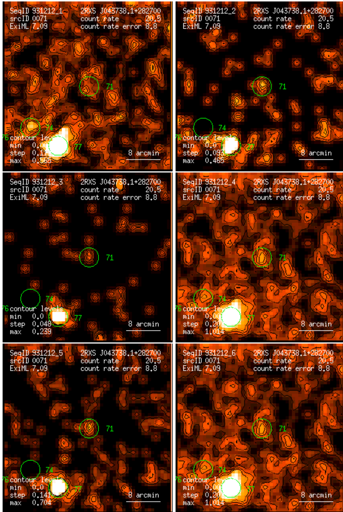
Figure 71: RASS 931212: detection 0071: band rate images, Gaussian filter: (1) PSPC channels 11 – 41, (2) 52 – 90, (3) 91 – 201, (4) 11 – 235, (5) 52 – 201, (6) 11 – 201. Broad band rates in counts/ks. Band rate contour levels in counts/ks/arcmin 2 .
