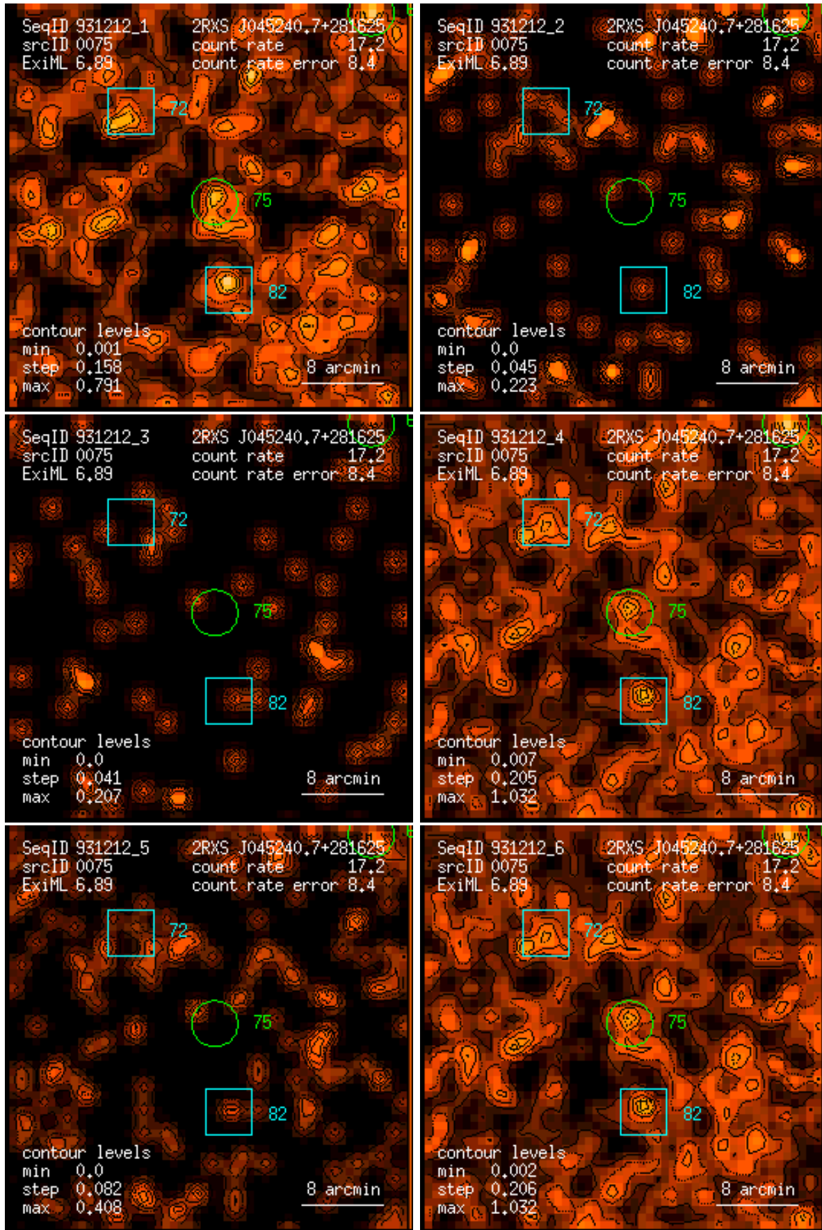
Figure 75: RASS 931212: detection 0075: band rate images, Gaussian filter: (1) PSPC channels 11 – 41, (2) 52 – 90, (3) 91 – 201, (4) 11 – 235, (5) 52 – 201, (6) 11 – 201. Broad band rates in counts/ks. Band rate contour levels in counts/ks/arcmin 2 .
