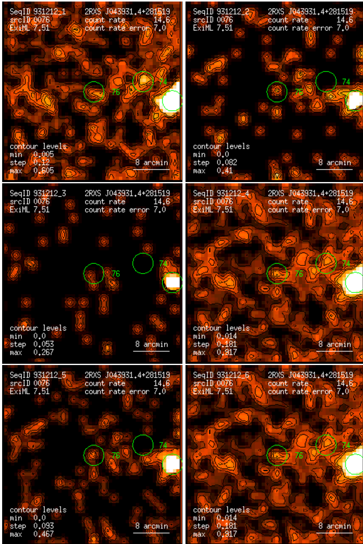
Figure 76: RASS 931212: detection 0076: band rate images, Gaussian filter: (1) PSPC channels 11 – 41, (2) 52 – 90, (3) 91 – 201, (4) 11 – 235, (5) 52 – 201, (6) 11 – 201. Broad band rates in counts/ks. Band rate contour levels in counts/ks/arcmin 2 .
