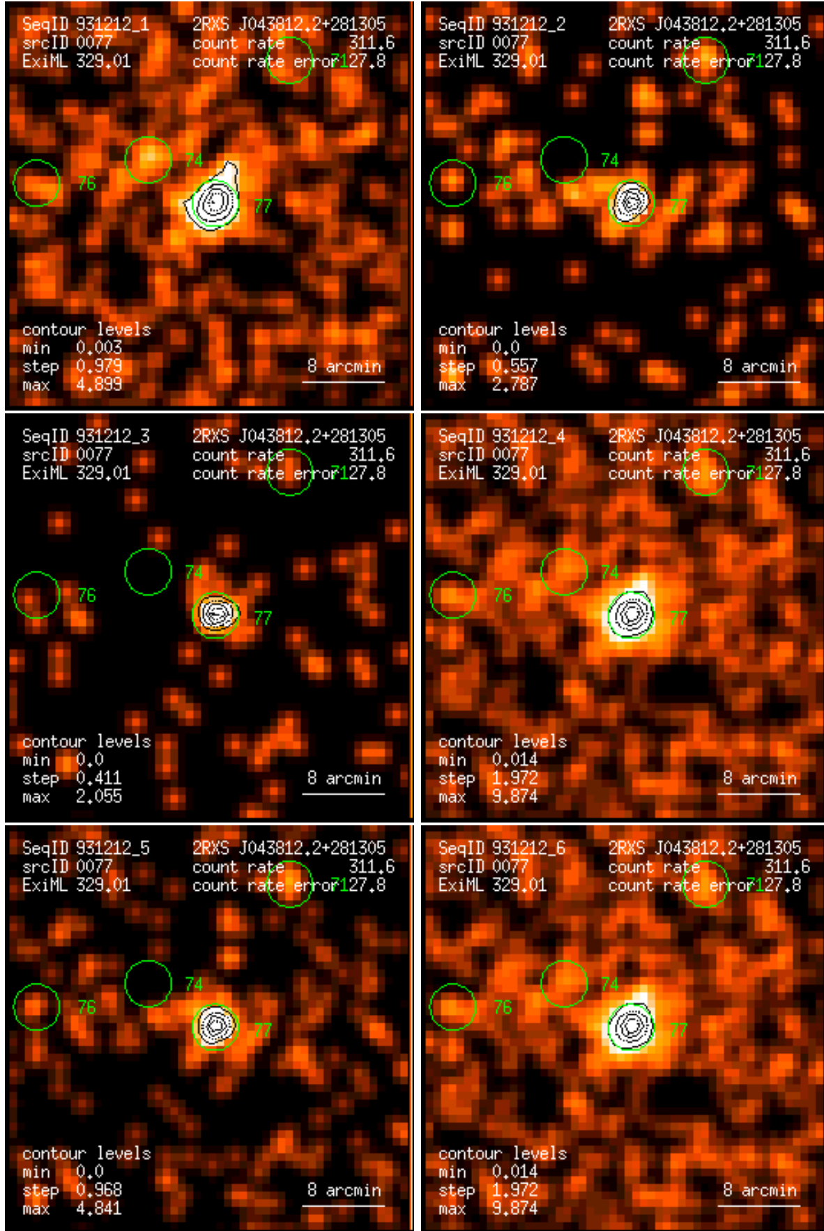
Figure 77: RASS 931212: detection 0077: band rate images, Gaussian filter: (1) PSPC channels 11 – 41, (2) 52 – 90, (3) 91 – 201, (4) 11 – 235, (5) 52 – 201, (6) 11 – 201. Broad band rates in counts/ks. Band rate contour levels in counts/ks/arcmin 2 .
