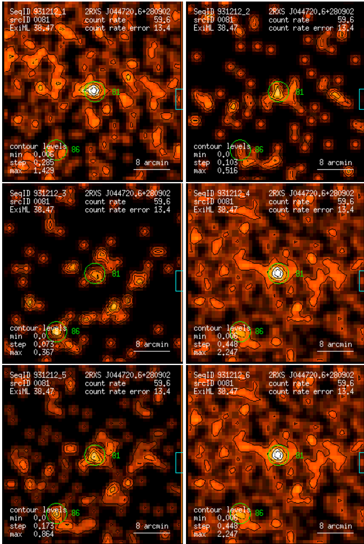
Figure 81: RASS 931212: detection 0081: band rate images, Gaussian filter: (1) PSPC channels 11 – 41, (2) 52 – 90, (3) 91 – 201, (4) 11 – 235, (5) 52 – 201, (6) 11 – 201. Broad band rates in counts/ks. Band rate contour levels in counts/ks/arcmin 2 .
