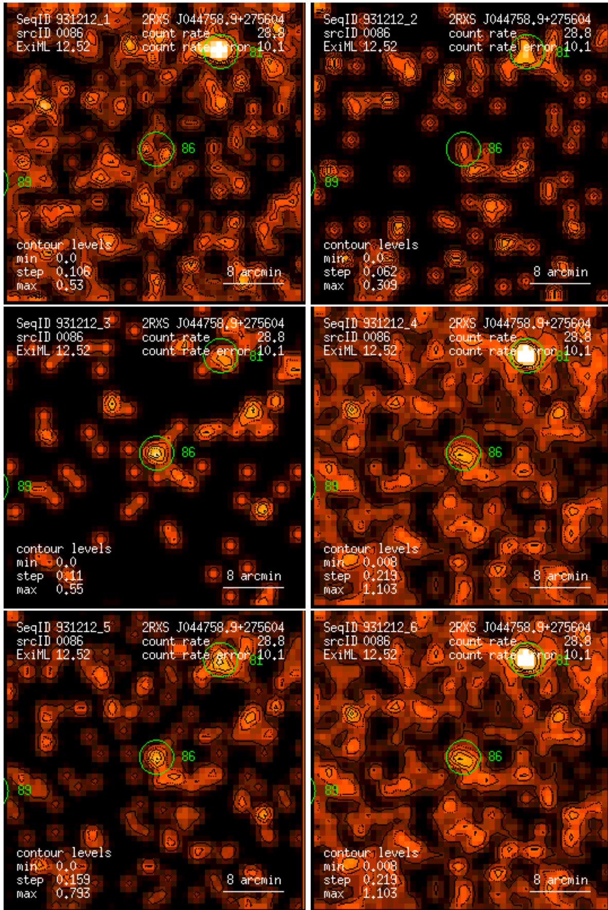
Figure 86: RASS 931212: detection 0086: band rate images, Gaussian filter: (1) PSPC channels 11 – 41, (2) 52 – 90, (3) 91 – 201, (4) 11 – 235, (5) 52 – 201, (6) 11 – 201. Broad band rates in counts/ks. Band rate contour levels in counts/ks/arcmin 2 .
