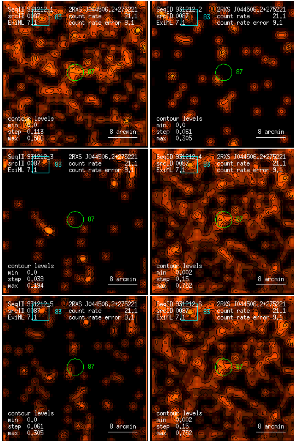
Figure 87: RASS 931212: detection 0087: band rate images, Gaussian filter: (1) PSPC channels 11 – 41, (2) 52 – 90, (3) 91 – 201, (4) 11 – 235, (5) 52 – 201, (6) 11 – 201. Broad band rates in counts/ks. Band rate contour levels in counts/ks/arcmin 2 .
