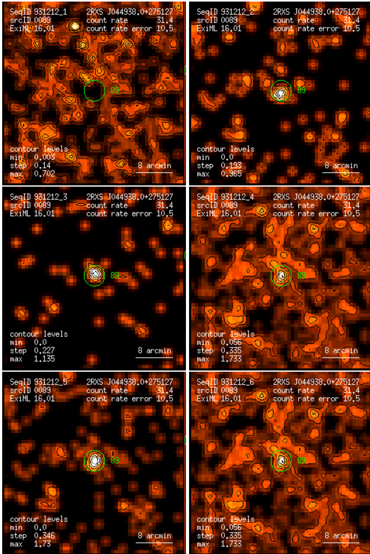
Figure 89: RASS 931212: detection 0089: band rate images, Gaussian filter: (1) PSPC channels 11 – 41, (2) 52 – 90, (3) 91 – 201, (4) 11 – 235, (5) 52 – 201, (6) 11 – 201. Broad band rates in counts/ks. Band rate contour levels in counts/ks/arcmin 2 .
