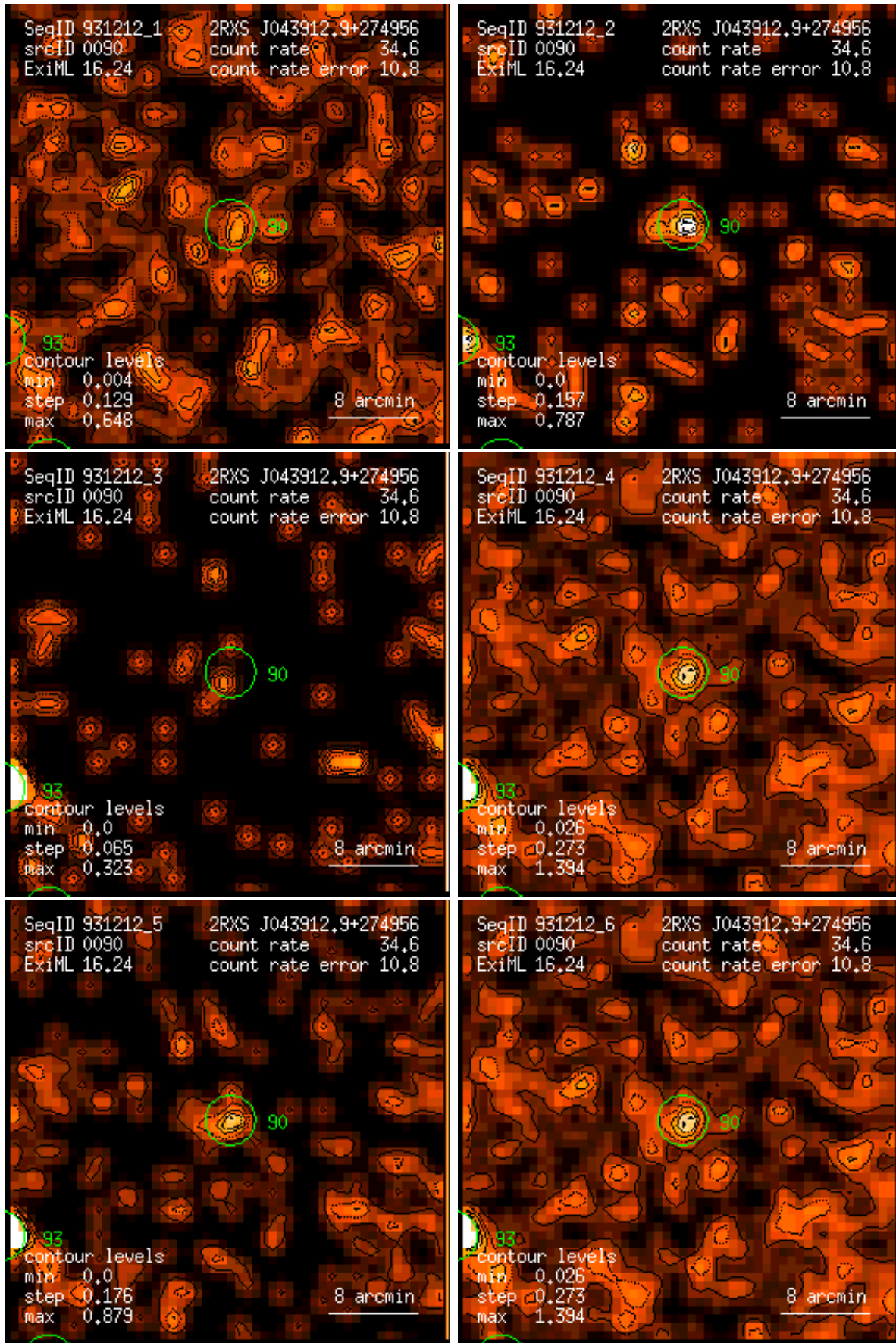
Figure 90: RASS 931212: detection 0090: band rate images, Gaussian filter: (1) PSPC channels 11 – 41, (2) 52 – 90, (3) 91 – 201, (4) 11 – 235, (5) 52 – 201, (6) 11 – 201. Broad band rates in counts/ks. Band rate contour levels in counts/ks/arcmin 2 .
