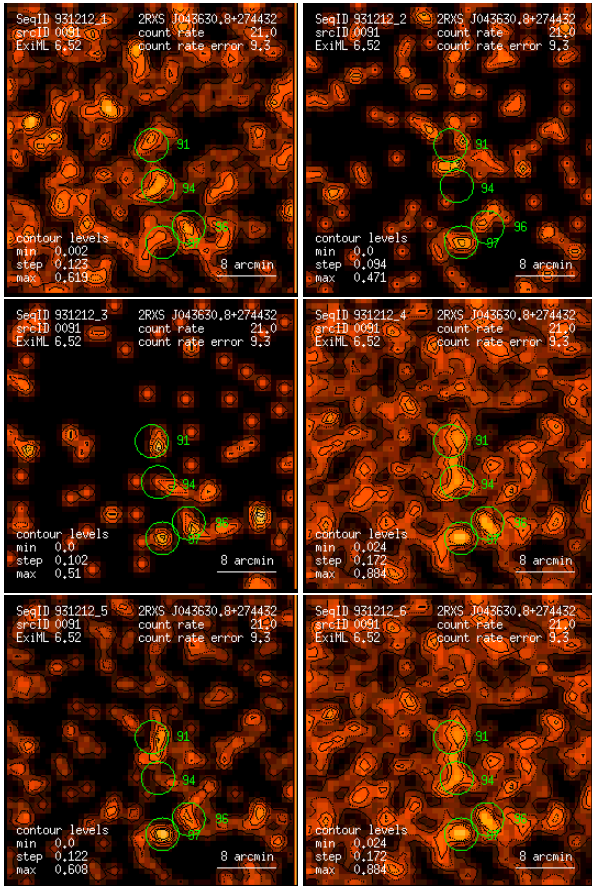
Figure 91: RASS 931212: detection 0091: band rate images, Gaussian filter: (1) PSPC channels 11 – 41, (2) 52 – 90, (3) 91 – 201, (4) 11 – 235, (5) 52 – 201, (6) 11 – 201. Broad band rates in counts/ks. Band rate contour levels in counts/ks/arcmin 2 .
