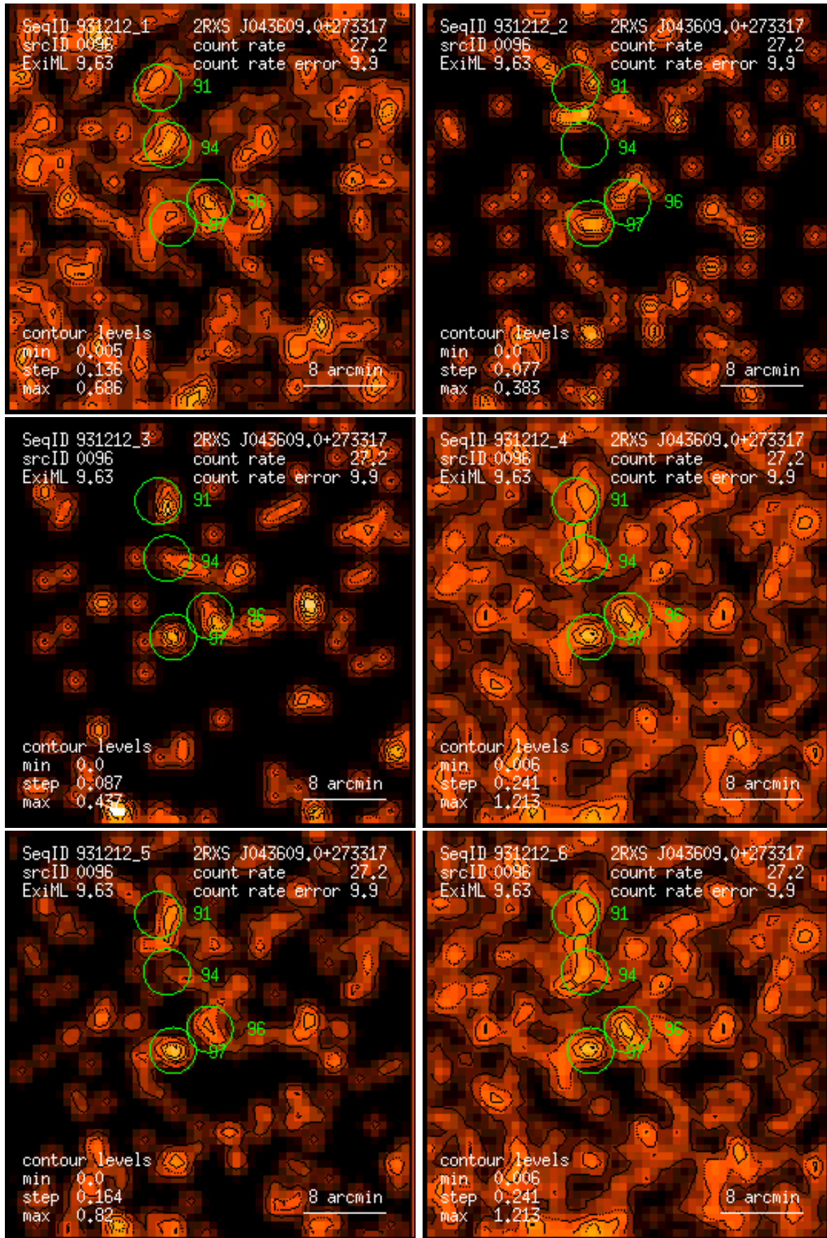
Figure 96: RASS 931212: detection 0096: band rate images, Gaussian filter: (1) PSPC channels 11 – 41, (2) 52 – 90, (3) 91 – 201, (4) 11 – 235, (5) 52 – 201, (6) 11 – 201. Broad band rates in counts/ks. Band rate contour levels in counts/ks/arcmin 2 .
