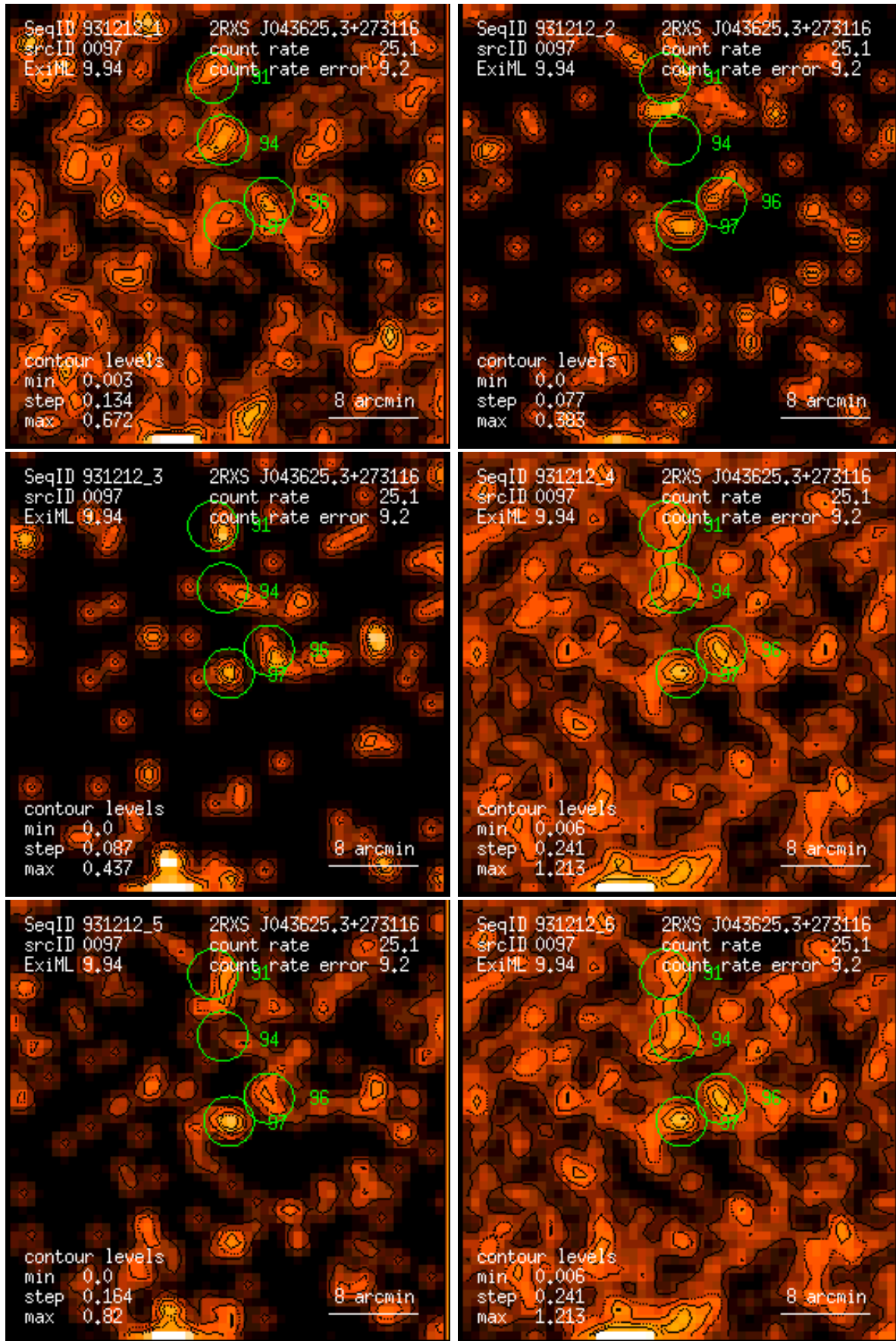
Figure 97: RASS 931212: detection 0097: band rate images, Gaussian filter: (1) PSPC channels 11 – 41, (2) 52 – 90, (3) 91 – 201, (4) 11 – 235, (5) 52 – 201, (6) 11 – 201. Broad band rates in counts/ks. Band rate contour levels in counts/ks/arcmin 2 .
