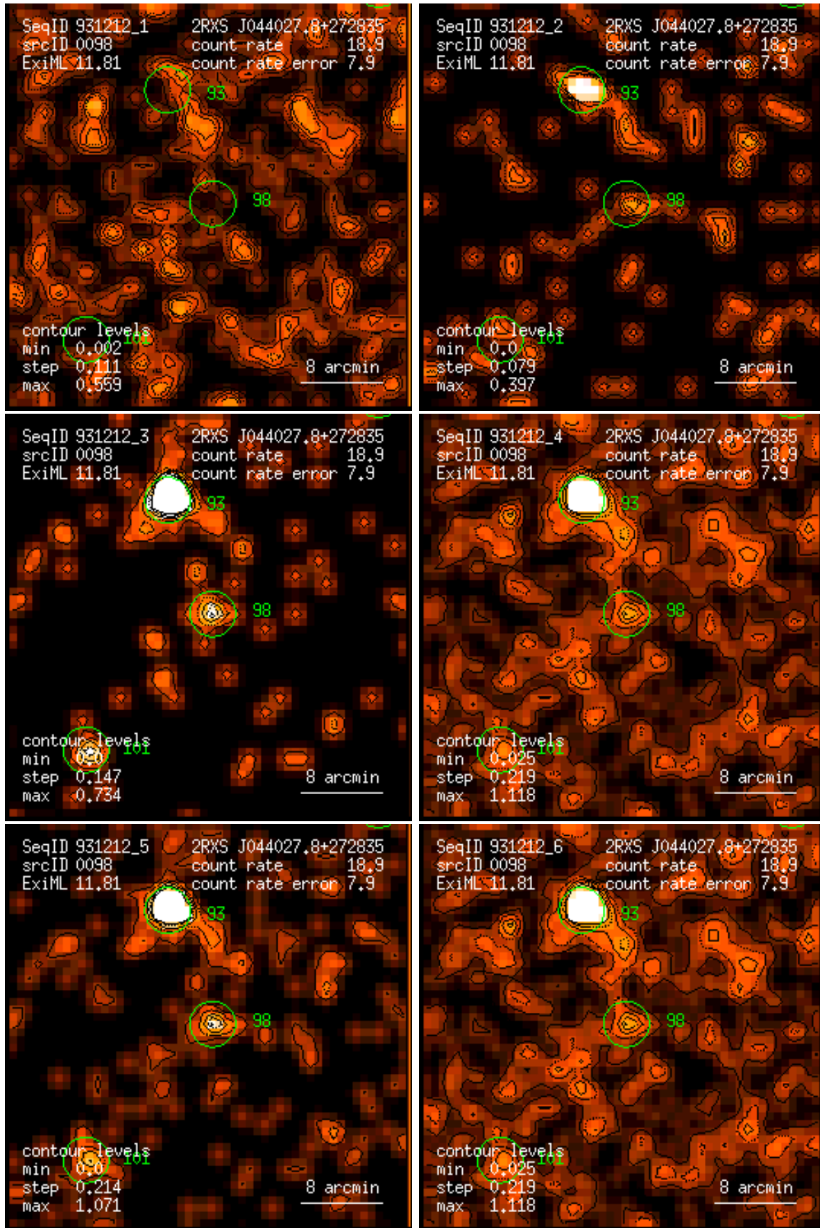
Figure 98: RASS 931212: detection 0098: band rate images, Gaussian filter: (1) PSPC channels 11 – 41, (2) 52 – 90, (3) 91 – 201, (4) 11 – 235, (5) 52 – 201, (6) 11 – 201. Broad band rates in counts/ks. Band rate contour levels in counts/ks/arcmin 2 .
