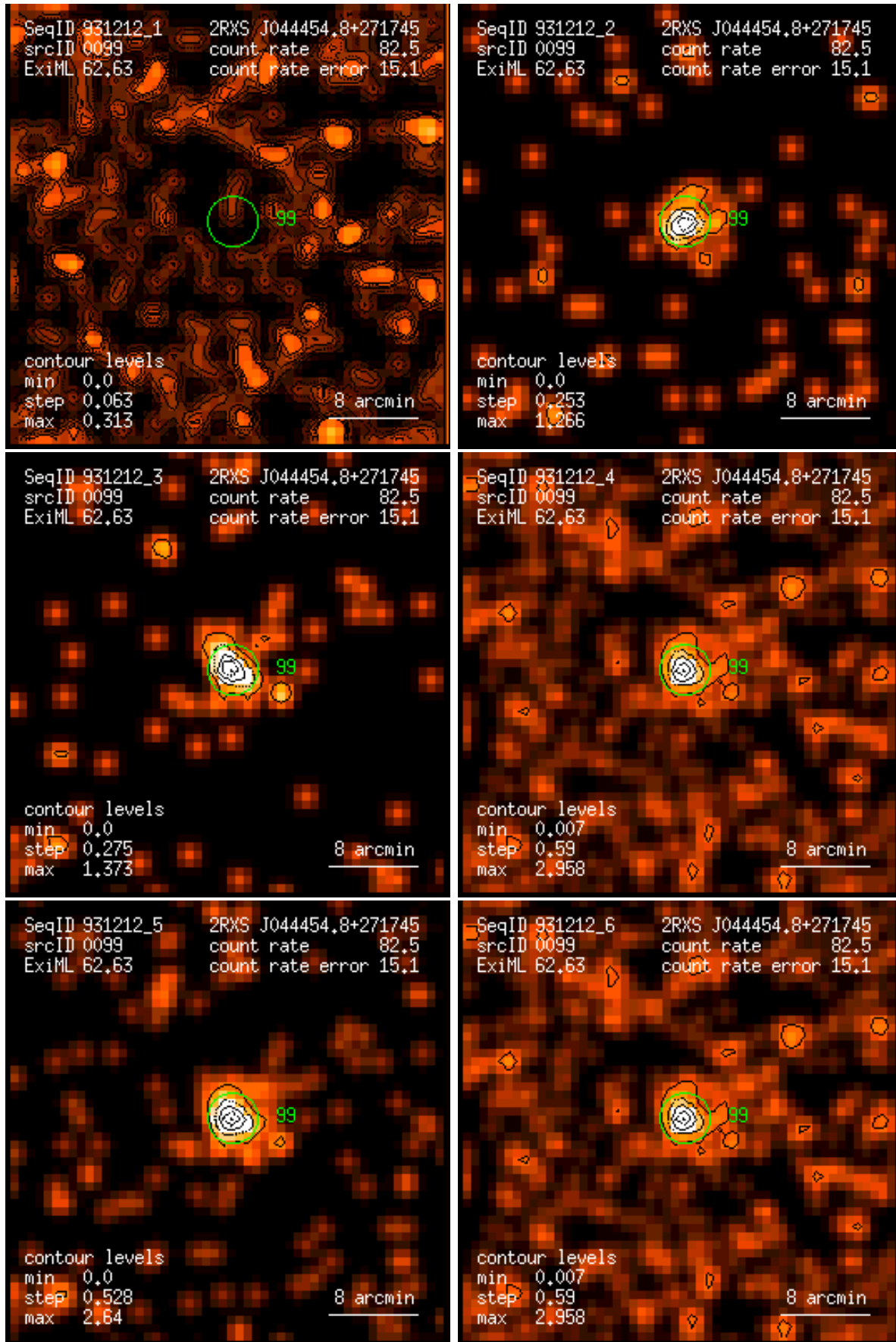
Figure 99: RASS 931212: detection 0099: band rate images, Gaussian filter: (1) PSPC channels 11 – 41, (2) 52 – 90, (3) 91 – 201, (4) 11 – 235, (5) 52 – 201, (6) 11 – 201. Broad band rates in counts/ks. Band rate contour levels in counts/ks/arcmin 2 .
