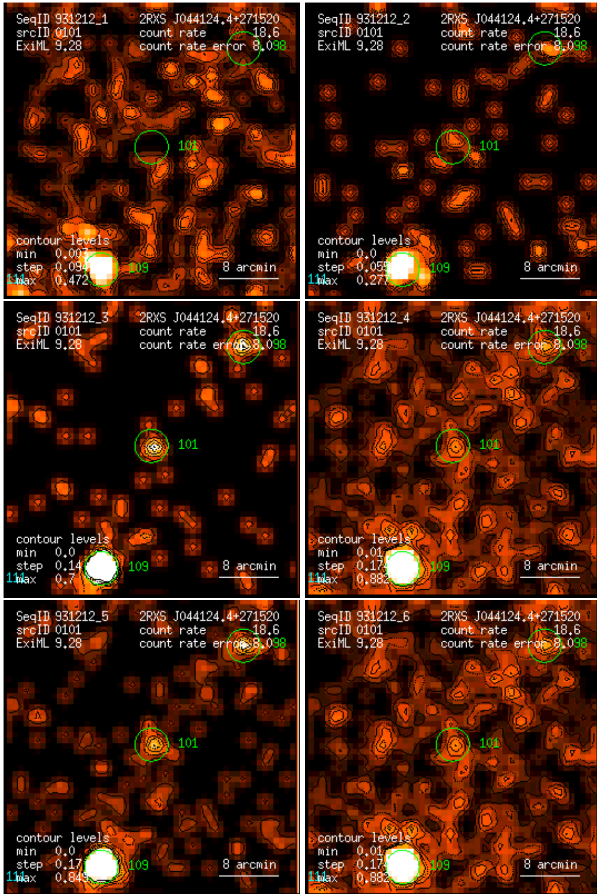
Figure 101: RASS 931212: detection 0101: band rate images, Gaussian filter: (1) PSPC channels 11 – 41, (2) 52 – 90, (3) 91 – 201, (4) 11 – 235, (5) 52 – 201, (6) 11 – 201. Broad band rates in counts/ks. Band rate contour levels in counts/ks/arcmin 2 .
