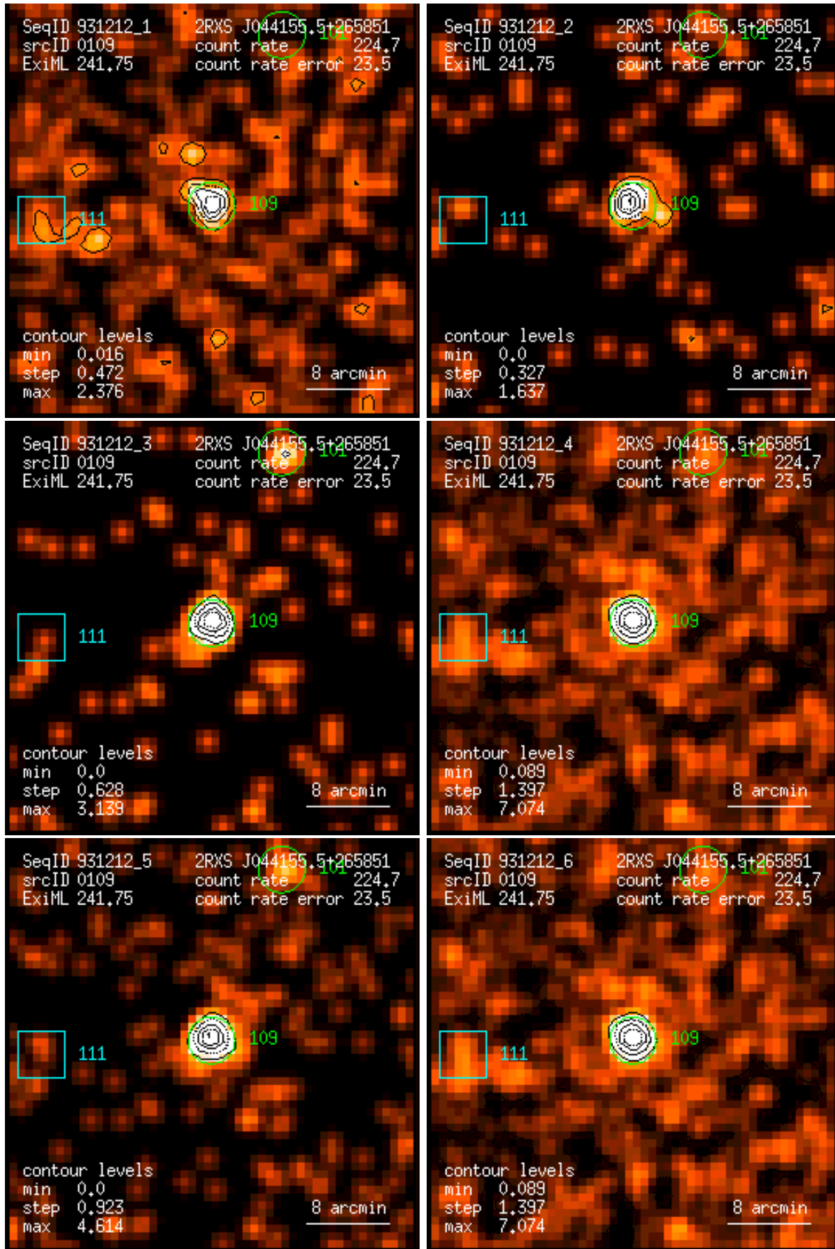
Figure 109: RASS 931212: detection 0109: band rate images, Gaussian filter: (1) PSPC channels 11 – 41, (2) 52 – 90, (3) 91 – 201, (4) 11 – 235, (5) 52 – 201, (6) 11 – 201. Broad band rates in counts/ks. Band rate contour levels in counts/ks/arcmin 2 .
