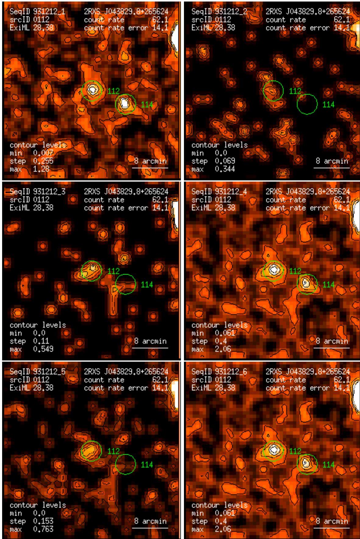
Figure 112: RASS 931212: detection 0112: band rate images, Gaussian filter: (1) PSPC channels 11 – 41, (2) 52 – 90, (3) 91 – 201, (4) 11 – 235, (5) 52 – 201, (6) 11 – 201. Broad band rates in counts/ks. Band rate contour levels in counts/ks/arcmin 2 .
