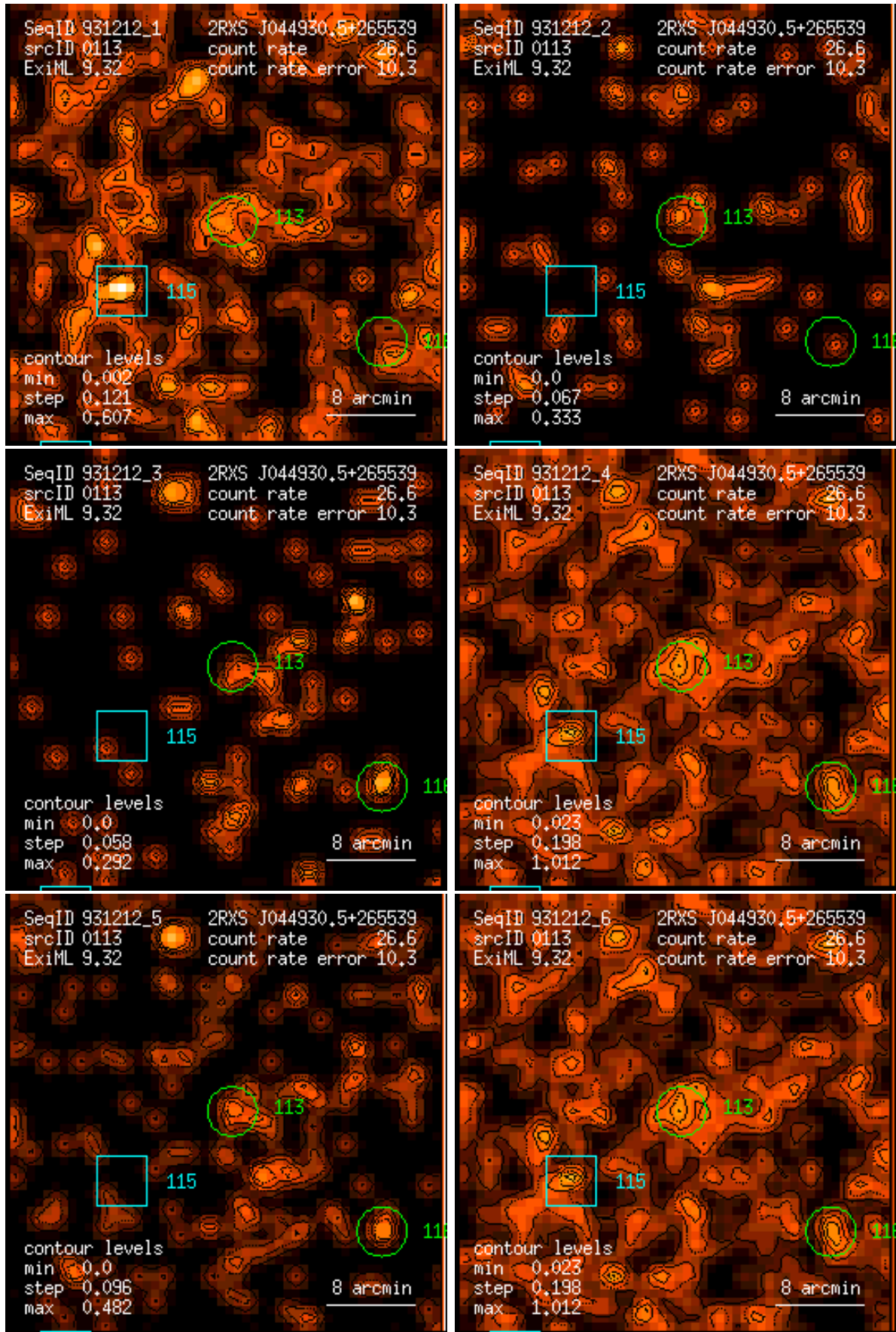
Figure 113: RASS 931212: detection 0113: band rate images, Gaussian filter: (1) PSPC channels 11 – 41, (2) 52 – 90, (3) 91 – 201, (4) 11 – 235, (5) 52 – 201, (6) 11 – 201. Broad band rates in counts/ks. Band rate contour levels in counts/ks/arcmin 2 .
