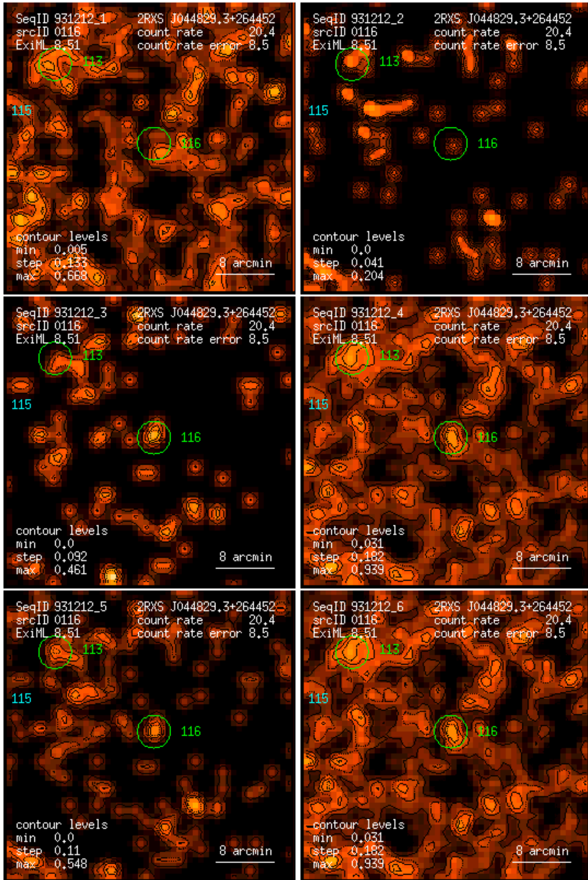
Figure 116: RASS 931212: detection 0116: band rate images, Gaussian filter: (1) PSPC channels 11 – 41, (2) 52 – 90, (3) 91 – 201, (4) 11 – 235, (5) 52 – 201, (6) 11 – 201. Broad band rates in counts/ks. Band rate contour levels in counts/ks/arcmin 2 .
