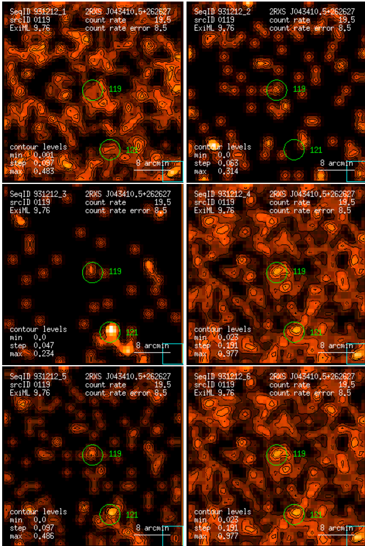
Figure 119: RASS 931212: detection 0119: band rate images, Gaussian filter: (1) PSPC channels 11 – 41, (2) 52 – 90, (3) 91 – 201, (4) 11 – 235, (5) 52 – 201, (6) 11 – 201. Broad band rates in counts/ks. Band rate contour levels in counts/ks/arcmin 2 .
