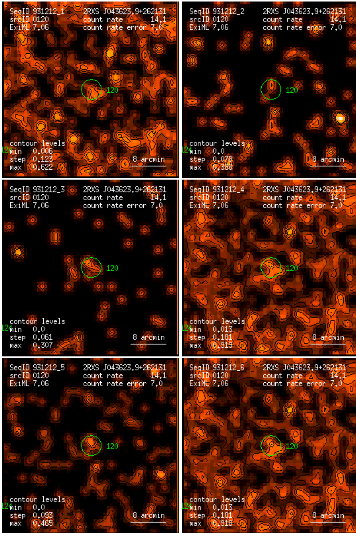
Figure 120: RASS 931212: detection 0120: band rate images, Gaussian filter: (1) PSPC channels 11 – 41, (2) 52 – 90, (3) 91 – 201, (4) 11 – 235, (5) 52 – 201, (6) 11 – 201. Broad band rates in counts/ks. Band rate contour levels in counts/ks/arcmin 2 .
