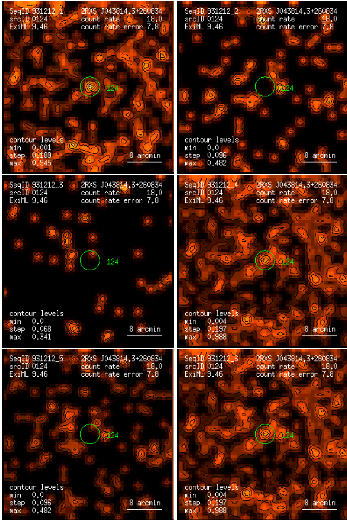
Figure 124: RASS 931212: detection 0124: band rate images, Gaussian filter: (1) PSPC channels 11 – 41, (2) 52 – 90, (3) 91 – 201, (4) 11 – 235, (5) 52 – 201, (6) 11 – 201. Broad band rates in counts/ks. Band rate contour levels in counts/ks/arcmin 2 .
