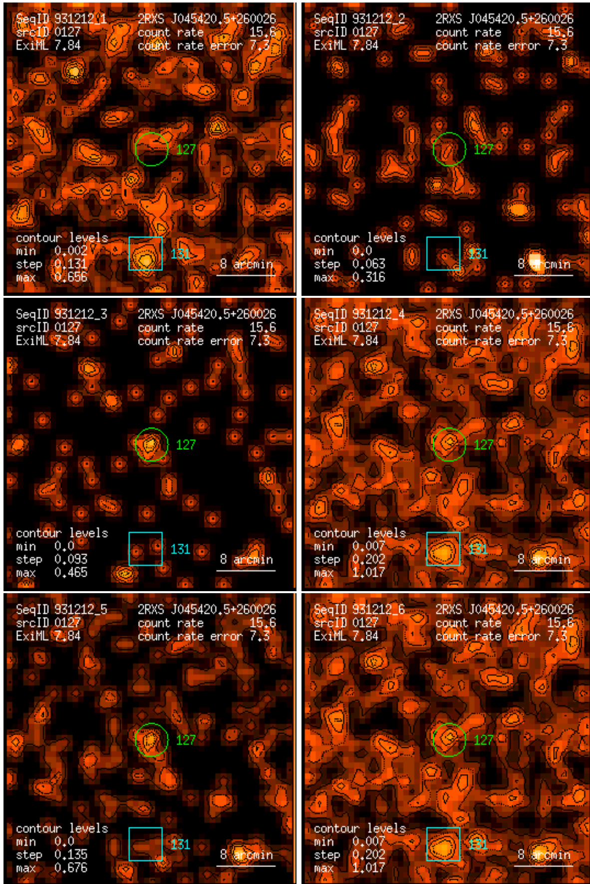
Figure 127: RASS 931212: detection 0127: band rate images, Gaussian filter: (1) PSPC channels 11 – 41, (2) 52 – 90, (3) 91 – 201, (4) 11 – 235, (5) 52 – 201, (6) 11 – 201. Broad band rates in counts/ks. Band rate contour levels in counts/ks/arcmin 2 .
