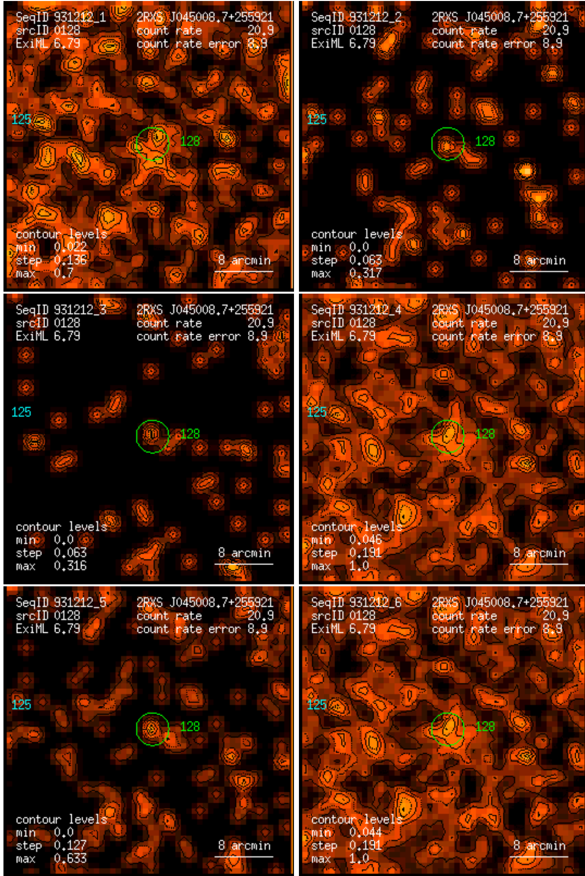
Figure 128: RASS 931212: detection 0128: band rate images, Gaussian filter: (1) PSPC channels 11 – 41, (2) 52 – 90, (3) 91 – 201, (4) 11 – 235, (5) 52 – 201, (6) 11 – 201. Broad band rates in counts/ks. Band rate contour levels in counts/ks/arcmin 2 .
