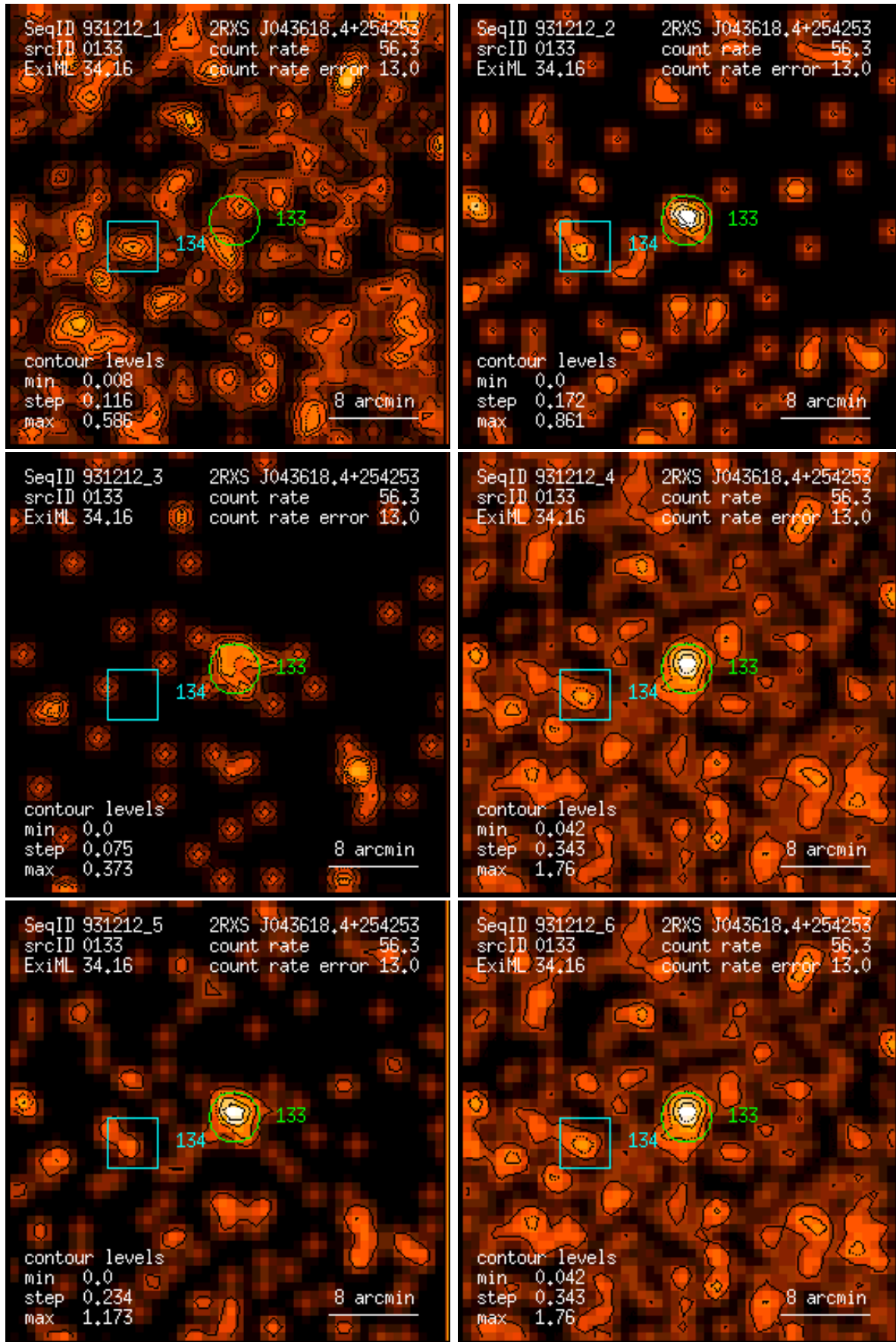
Figure 133: RASS 931212: detection 0133: band rate images, Gaussian filter: (1) PSPC channels 11 – 41, (2) 52 – 90, (3) 91 – 201, (4) 11 – 235, (5) 52 – 201, (6) 11 – 201. Broad band rates in counts/ks. Band rate contour levels in counts/ks/arcmin 2 .
