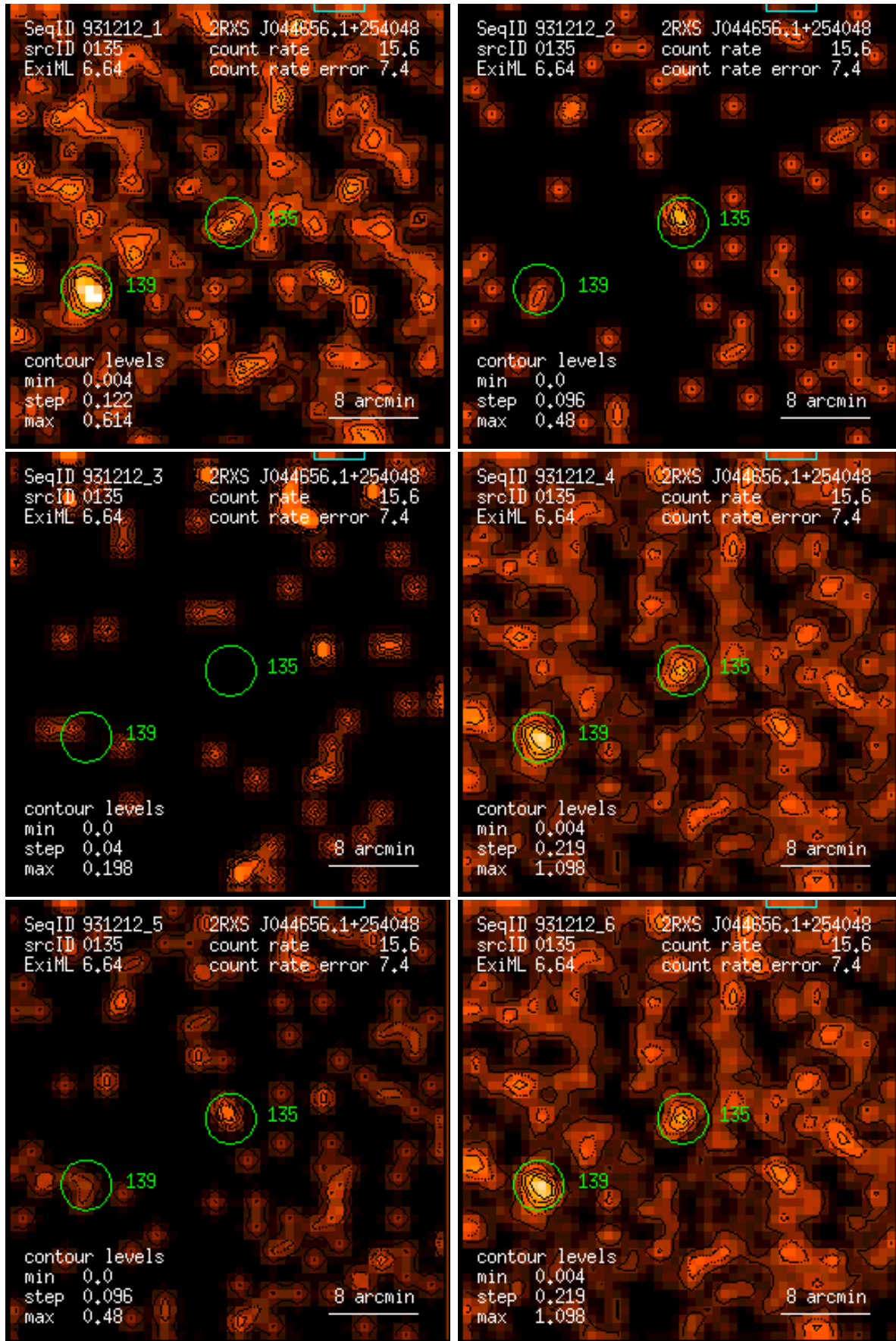
Figure 135: RASS 931212: detection 0135: band rate images, Gaussian filter: (1) PSPC channels 11 – 41, (2) 52 – 90, (3) 91 – 201, (4) 11 – 235, (5) 52 – 201, (6) 11 – 201. Broad band rates in counts/ks. Band rate contour levels in counts/ks/arcmin 2 .
