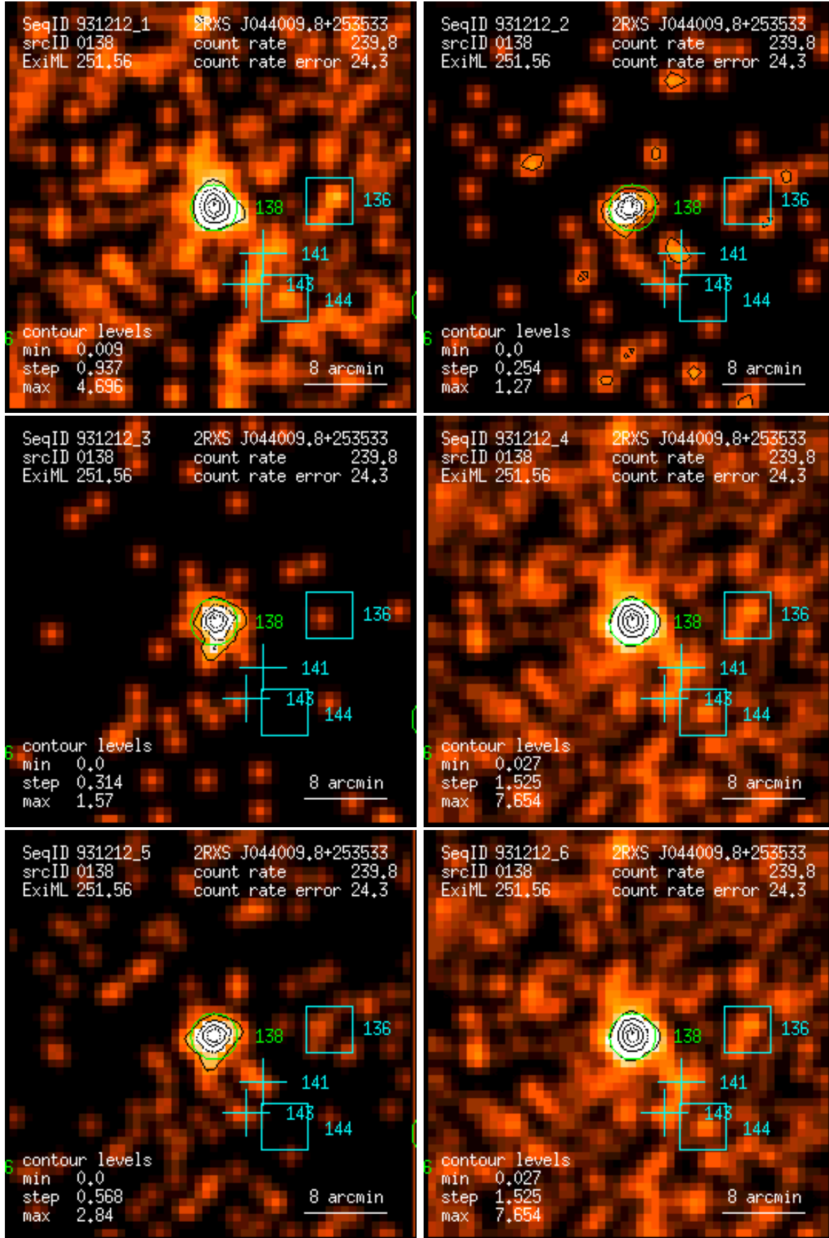
Figure 138: RASS 931212: detection 0138: band rate images, Gaussian filter: (1) PSPC channels 11 – 41, (2) 52 – 90, (3) 91 – 201, (4) 11 – 235, (5) 52 – 201, (6) 11 – 201. Broad band rates in counts/ks. Band rate contour levels in counts/ks/arcmin 2 .
