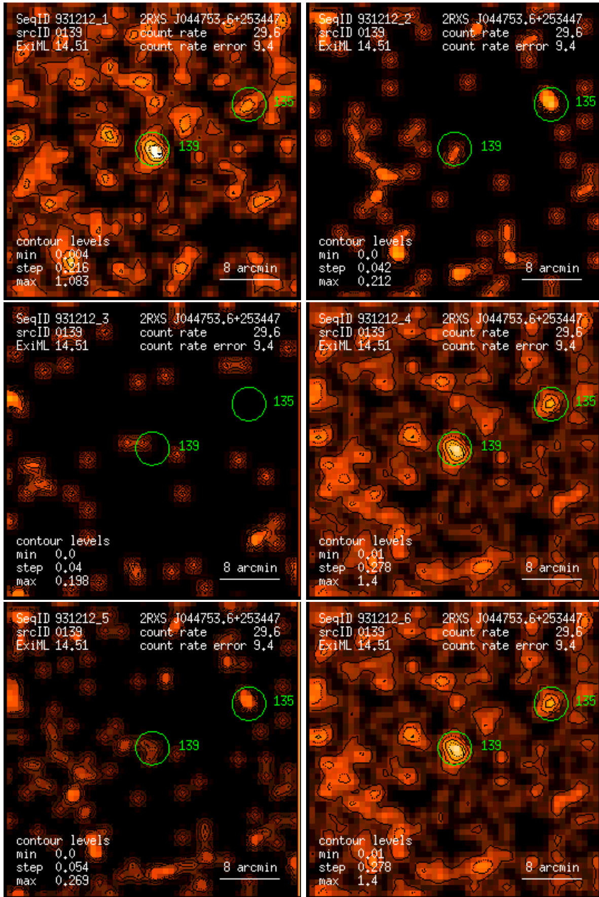
Figure 139: RASS 931212: detection 0139: band rate images, Gaussian filter: (1) PSPC channels 11 – 41, (2) 52 – 90, (3) 91 – 201, (4) 11 – 235, (5) 52 – 201, (6) 11 – 201. Broad band rates in counts/ks. Band rate contour levels in counts/ks/arcmin 2 .
