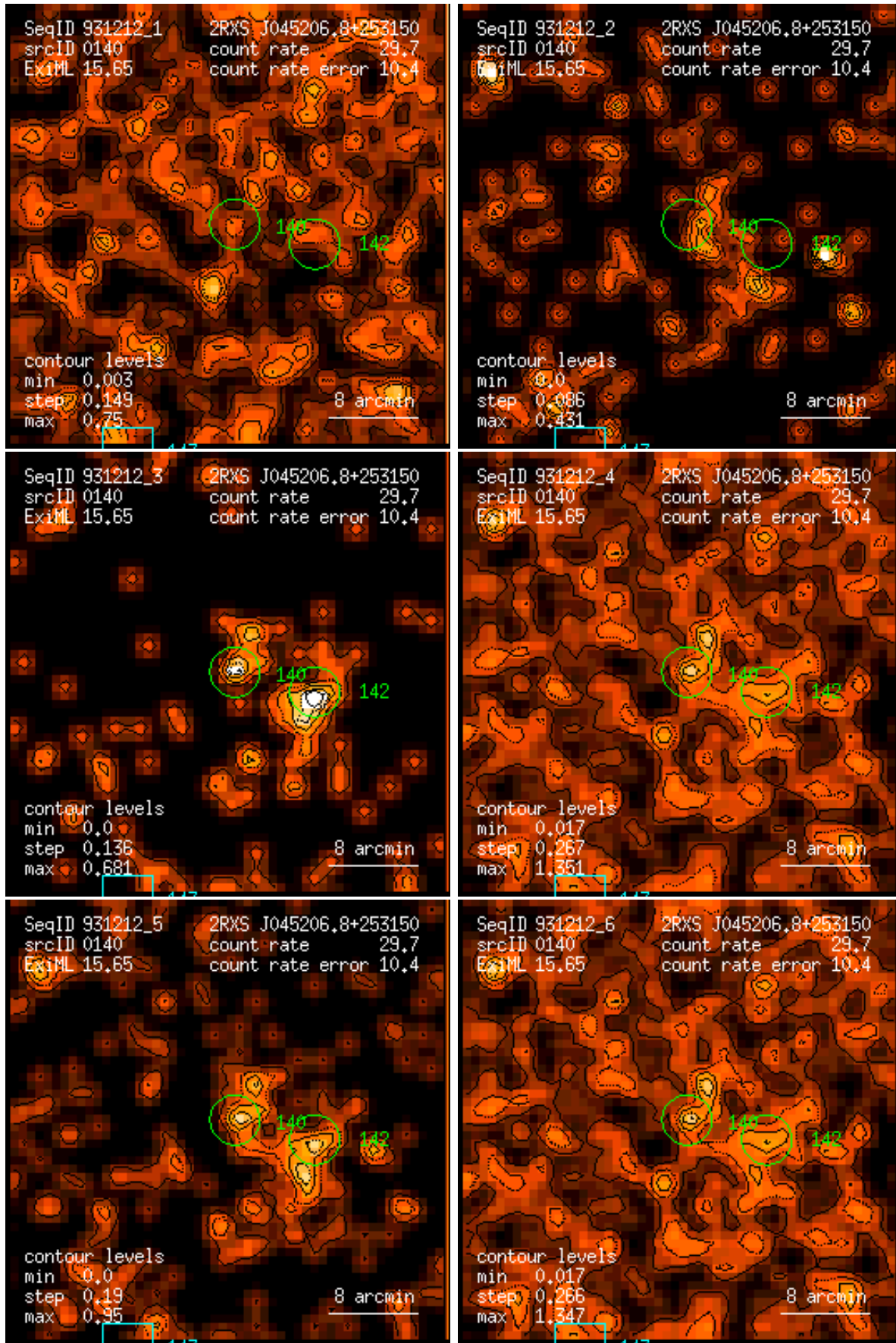
Figure 140: RASS 931212: detection 0140: band rate images, Gaussian filter: (1) PSPC channels 11 – 41, (2) 52 – 90, (3) 91 – 201, (4) 11 – 235, (5) 52 – 201, (6) 11 – 201. Broad band rates in counts/ks. Band rate contour levels in counts/ks/arcmin 2 .
