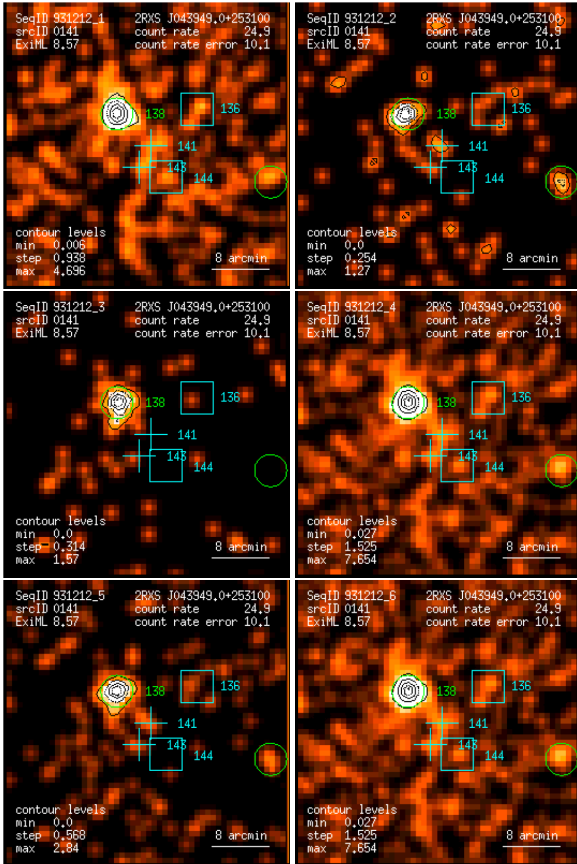
Figure 141: RASS 931212: detection 0141: band rate images, Gaussian filter: (1) PSPC channels 11 – 41, (2) 52 – 90, (3) 91 – 201, (4) 11 – 235, (5) 52 – 201, (6) 11 – 201. Broad band rates in counts/ks. Band rate contour levels in counts/ks/arcmin 2 .
