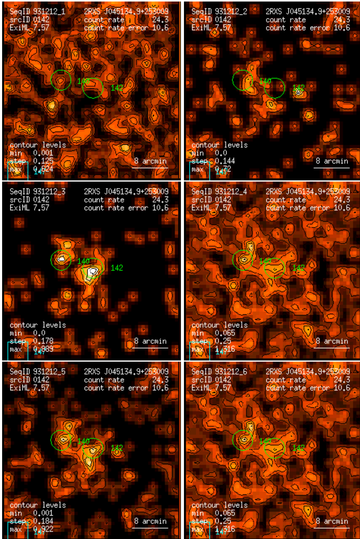
Figure 142: RASS 931212: detection 0142: band rate images, Gaussian filter: (1) PSPC channels 11 – 41, (2) 52 – 90, (3) 91 – 201, (4) 11 – 235, (5) 52 – 201, (6) 11 – 201. Broad band rates in counts/ks. Band rate contour levels in counts/ks/arcmin 2 .
