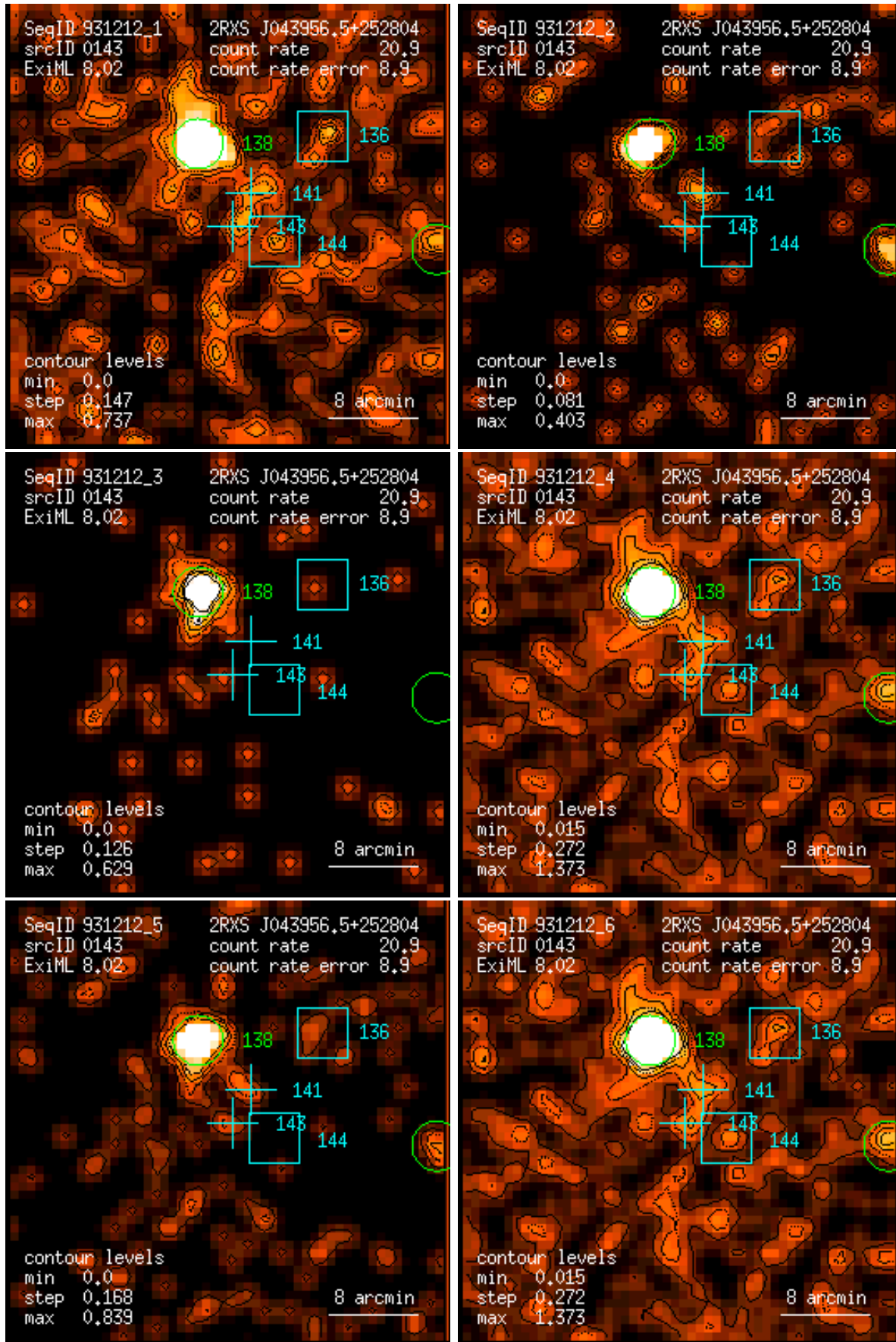
Figure 143: RASS 931212: detection 0143: band rate images, Gaussian filter: (1) PSPC channels 11 – 41, (2) 52 – 90, (3) 91 – 201, (4) 11 – 235, (5) 52 – 201, (6) 11 – 201. Broad band rates in counts/ks. Band rate contour levels in counts/ks/arcmin 2 .
