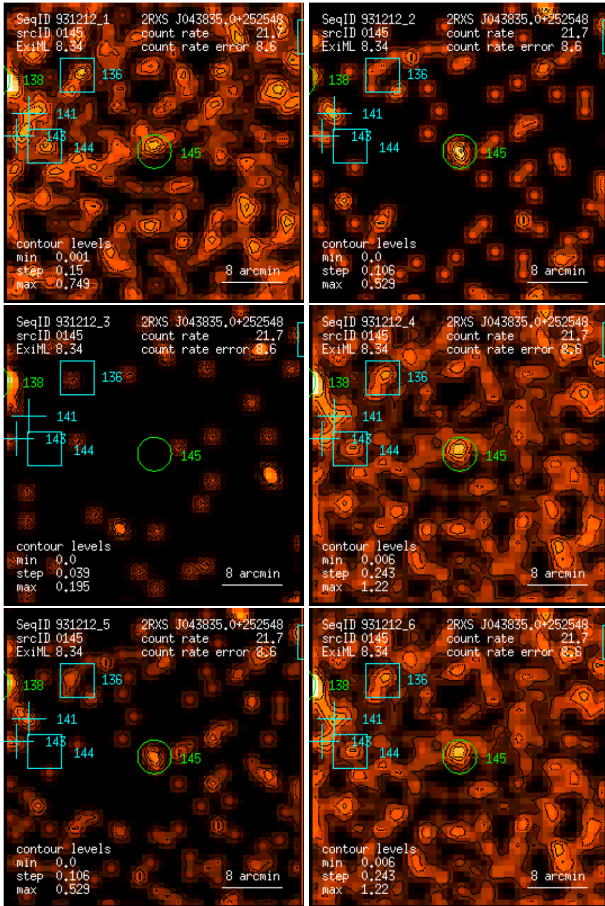
Figure 145: RASS 931212: detection 0145: band rate images, Gaussian filter: (1) PSPC channels 11 – 41, (2) 52 – 90, (3) 91 – 201, (4) 11 – 235, (5) 52 – 201, (6) 11 – 201. Broad band rates in counts/ks. Band rate contour levels in counts/ks/arcmin 2 .
