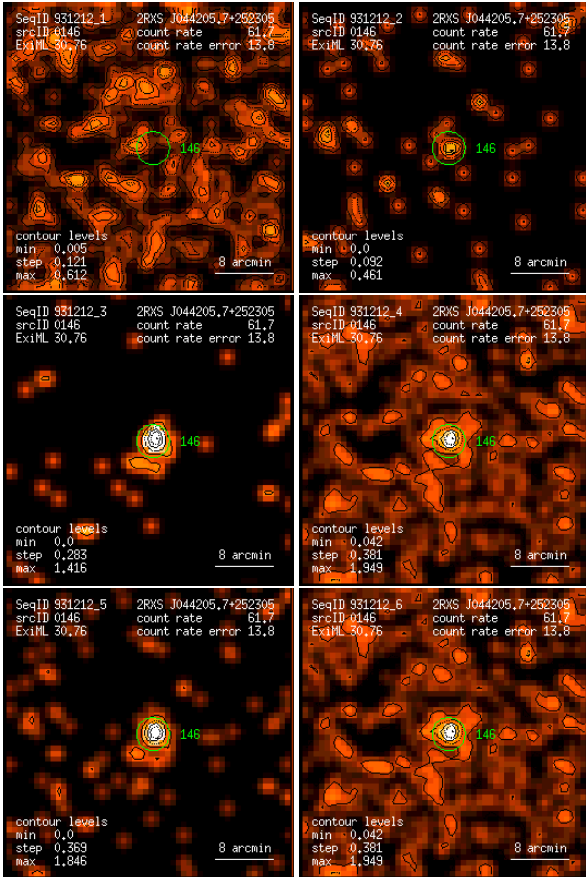
Figure 146: RASS 931212: detection 0146: band rate images, Gaussian filter: (1) PSPC channels 11 – 41, (2) 52 – 90, (3) 91 – 201, (4) 11 – 235, (5) 52 – 201, (6) 11 – 201. Broad band rates in counts/ks. Band rate contour levels in counts/ks/arcmin 2 .
