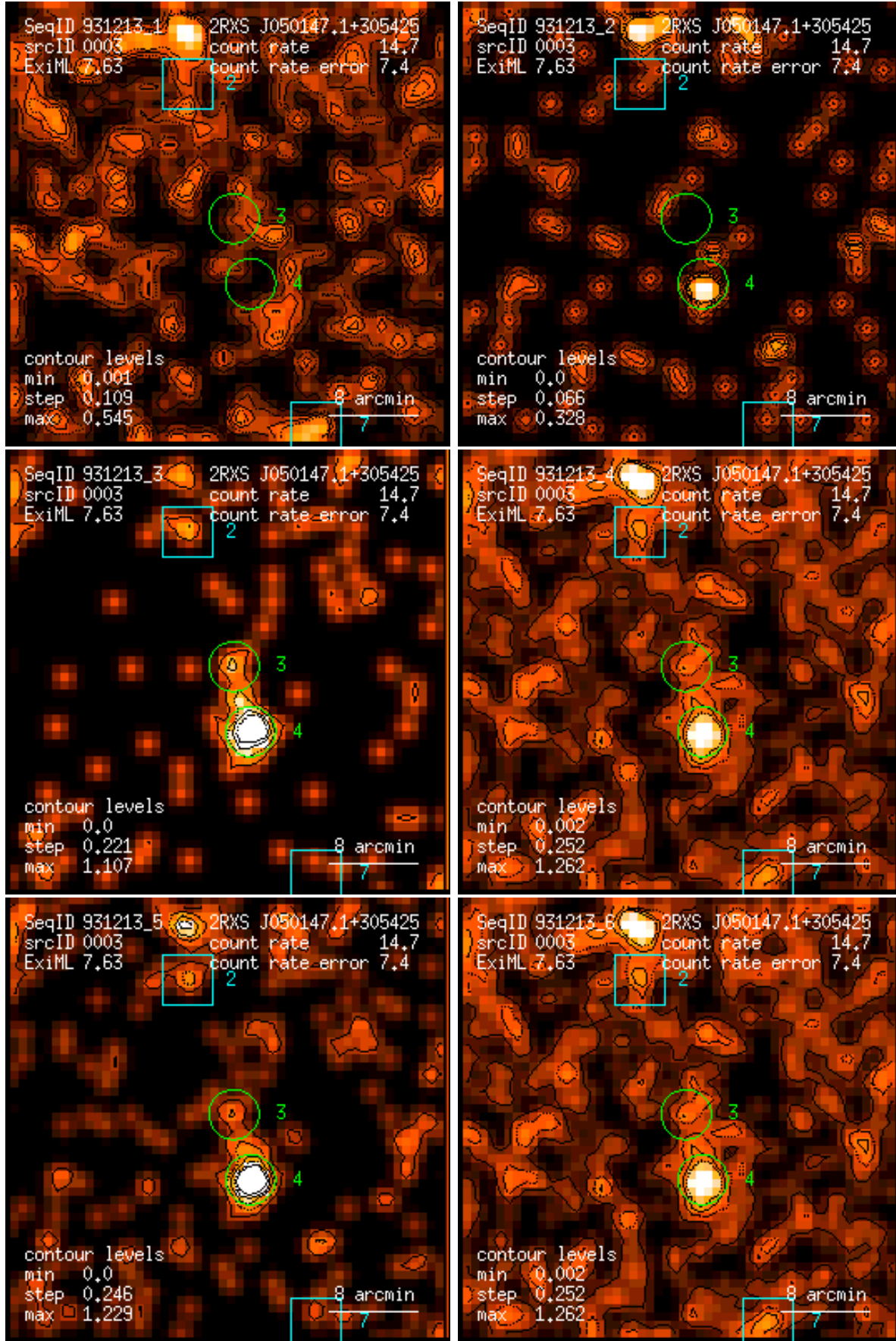
Figure 3: RASS 931213: detection 0003: band rate images, Gaussian filter: (1) PSPC channels 11 – 41, (2) 52 – 90, (3) 91 – 201, (4) 11 – 235, (5) 52 – 201, (6) 11 – 201. Broad band rates in counts/ks. Band rate contour levels in counts/ks/arcmin 2 .
