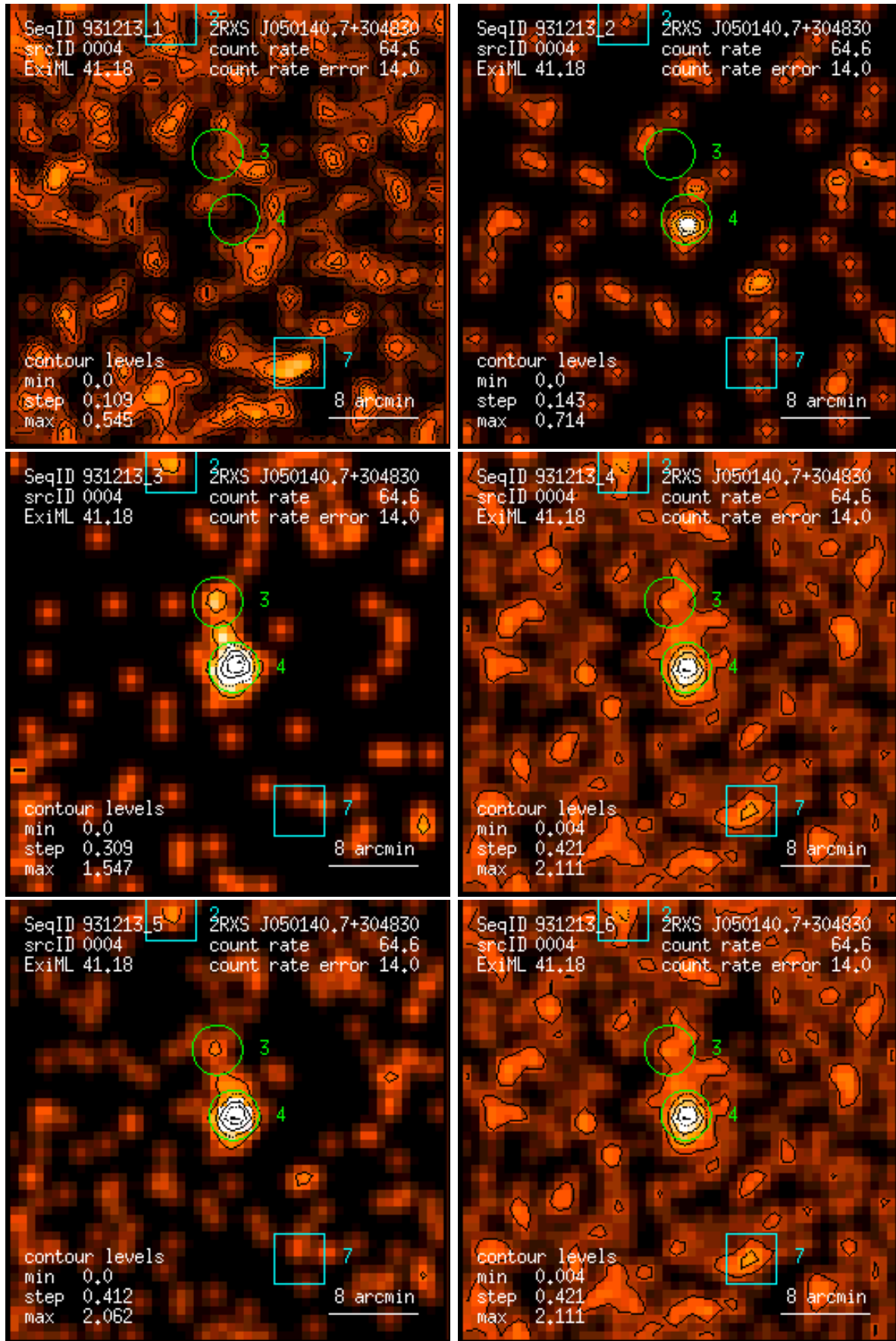
Figure 4: RASS 931213: detection 0004: band rate images, Gaussian filter: (1) PSPC channels 11 – 41, (2) 52 – 90, (3) 91 – 201, (4) 11 – 235, (5) 52 – 201, (6) 11 – 201. Broad band rates in counts/ks. Band rate contour levels in counts/ks/arcmin 2 .
