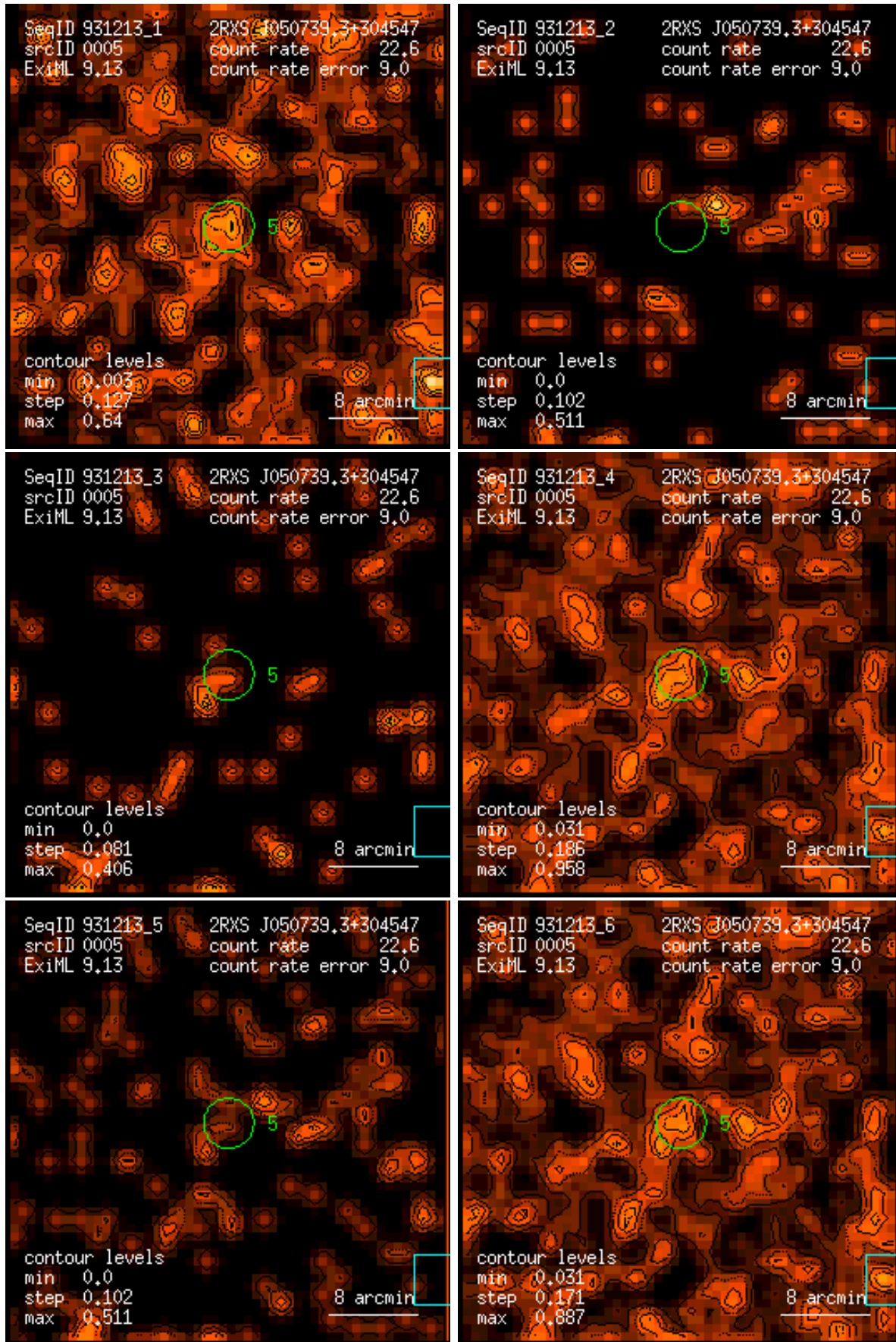
Figure 5: RASS 931213: detection 0005: band rate images, Gaussian filter: (1) PSPC channels 11 – 41, (2) 52 – 90, (3) 91 – 201, (4) 11 – 235, (5) 52 – 201, (6) 11 – 201. Broad band rates in counts/ks. Band rate contour levels in counts/ks/arcmin 2 .
