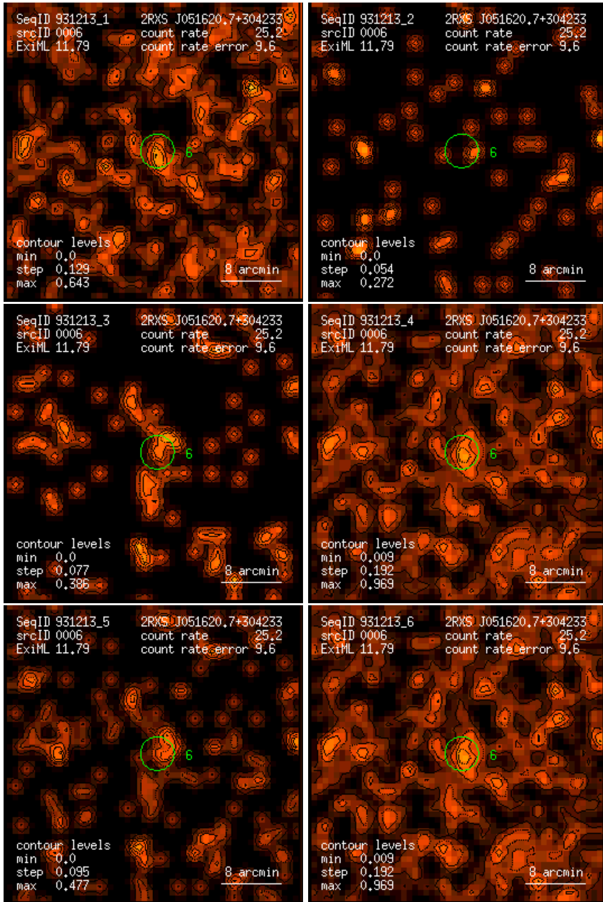
Figure 6: RASS 931213: detection 0006: band rate images, Gaussian filter: (1) PSPC channels 11 – 41, (2) 52 – 90, (3) 91 – 201, (4) 11 – 235, (5) 52 – 201, (6) 11 – 201. Broad band rates in counts/ks. Band rate contour levels in counts/ks/arcmin 2 .
