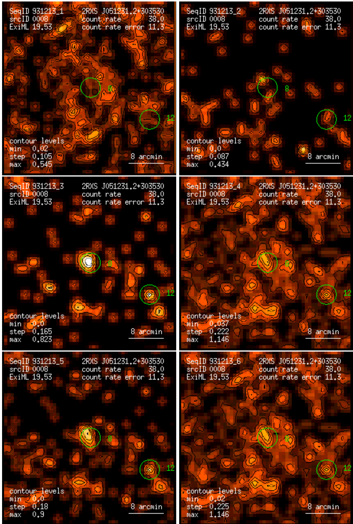
Figure 8: RASS 931213: detection 0008: band rate images, Gaussian filter: (1) PSPC channels 11 – 41, (2) 52 – 90, (3) 91 – 201, (4) 11 – 235, (5) 52 – 201, (6) 11 – 201. Broad band rates in counts/ks. Band rate contour levels in counts/ks/arcmin 2 .
