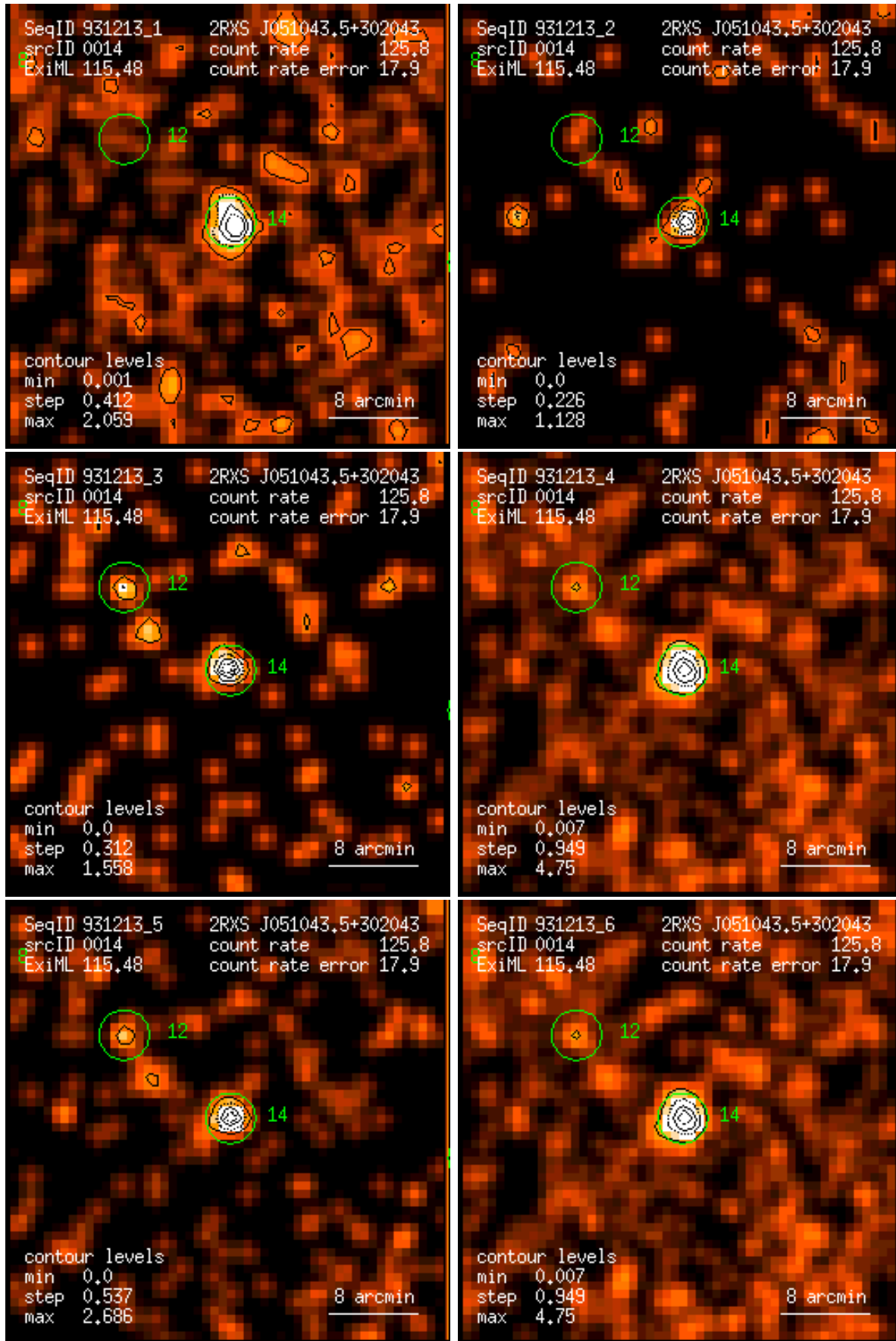
Figure 14: RASS 931213: detection 0014: band rate images, Gaussian filter: (1) PSPC channels 11 – 41, (2) 52 – 90, (3) 91 – 201, (4) 11 – 235, (5) 52 – 201, (6) 11 – 201. Broad band rates in counts/ks. Band rate contour levels in counts/ks/arcmin 2 .
