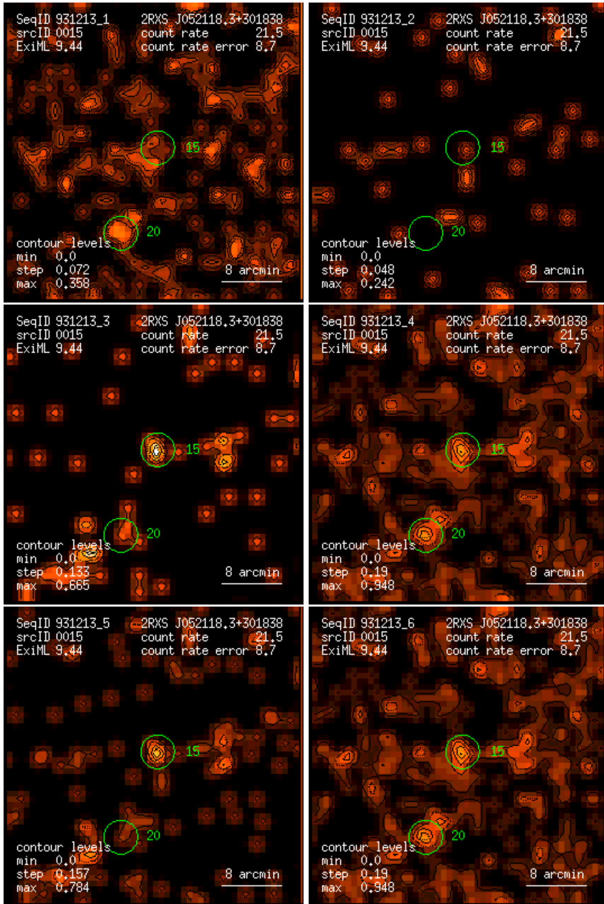
Figure 15: RASS 931213: detection 0015: band rate images, Gaussian filter: (1) PSPC channels 11 – 41, (2) 52 – 90, (3) 91 – 201, (4) 11 – 235, (5) 52 – 201, (6) 11 – 201. Broad band rates in counts/ks. Band rate contour levels in counts/ks/arcmin 2 .
