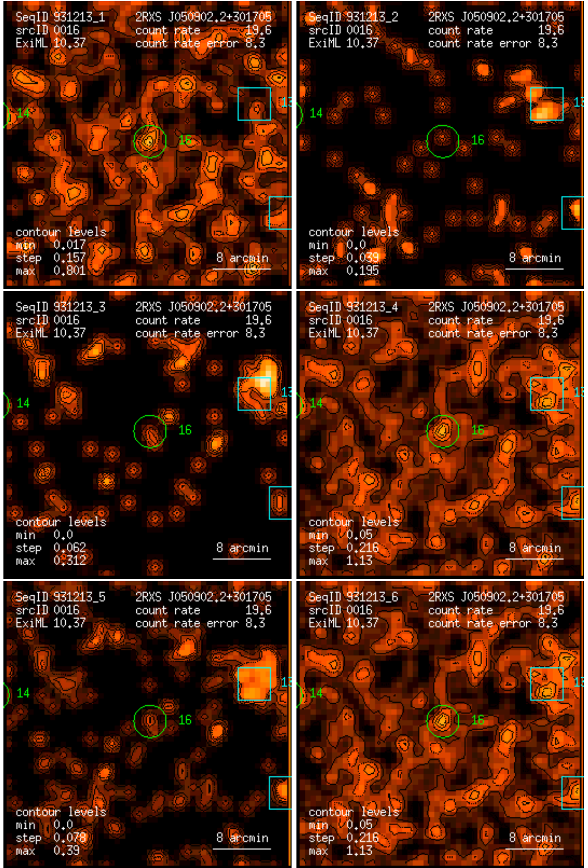
Figure 16: RASS 931213: detection 0016: band rate images, Gaussian filter: (1) PSPC channels 11 – 41, (2) 52 – 90, (3) 91 – 201, (4) 11 – 235, (5) 52 – 201, (6) 11 – 201. Broad band rates in counts/ks. Band rate contour levels in counts/ks/arcmin 2 .
