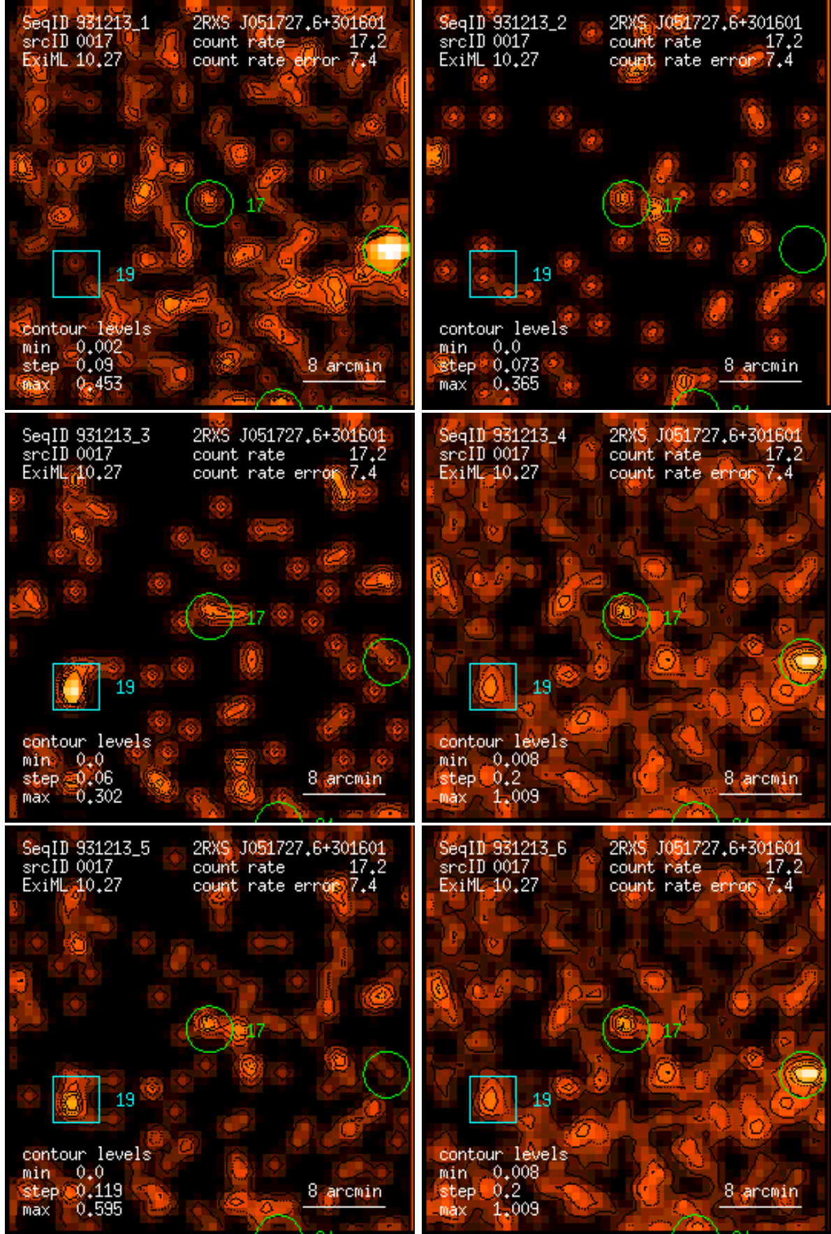
Figure 17: RASS 931213: detection 0017: band rate images, Gaussian filter: (1) PSPC channels 11 – 41, (2) 52 – 90, (3) 91 – 201, (4) 11 – 235, (5) 52 – 201, (6) 11 – 201. Broad band rates in counts/ks. Band rate contour levels in counts/ks/arcmin 2 .
