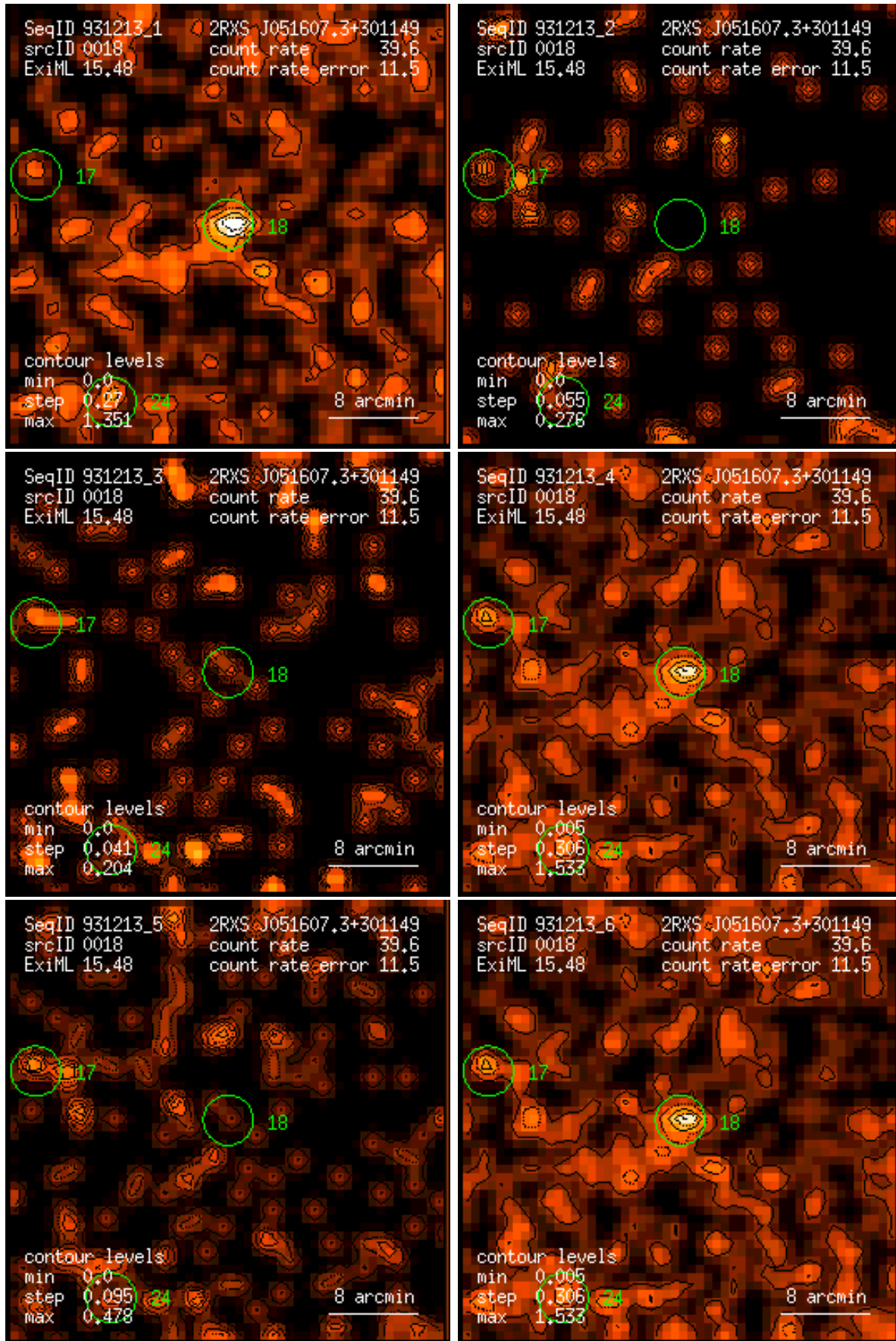
Figure 18: RASS 931213: detection 0018: band rate images, Gaussian filter: (1) PSPC channels 11 – 41, (2) 52 – 90, (3) 91 – 201, (4) 11 – 235, (5) 52 – 201, (6) 11 – 201. Broad band rates in counts/ks. Band rate contour levels in counts/ks/arcmin 2 .
