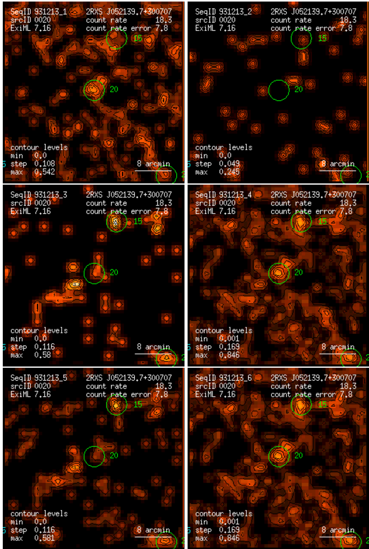
Figure 20: RASS 931213: detection 0020: band rate images, Gaussian filter: (1) PSPC channels 11 – 41, (2) 52 – 90, (3) 91 – 201, (4) 11 – 235, (5) 52 – 201, (6) 11 – 201. Broad band rates in counts/ks. Band rate contour levels in counts/ks/arcmin 2 .
