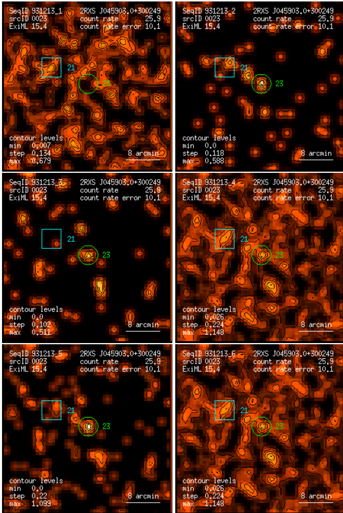
Figure 23: RASS 931213: detection 0023: band rate images, Gaussian filter: (1) PSPC channels 11 – 41, (2) 52 – 90, (3) 91 – 201, (4) 11 – 235, (5) 52 – 201, (6) 11 – 201. Broad band rates in counts/ks. Band rate contour levels in counts/ks/arcmin 2 .
